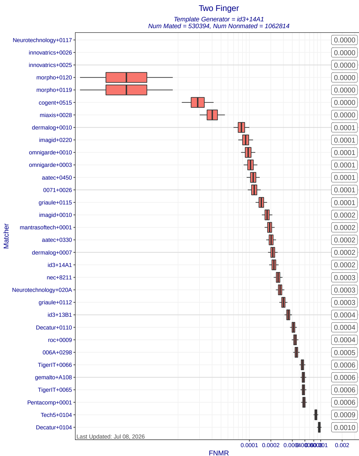
Figure 7: Two Finger FNMR at FMR=0.01 when different matchers compare templates created by template generator id3+14A1. Each box represents uncertainty about the true FNMR. The box edges mark the 50% confidence intervals while the whiskers mark the 90% confidence intervals. The numbers on the right show the actual computed FNMRs. Score-level fusion is achieved by averaging the scores for left and right index fingers.
