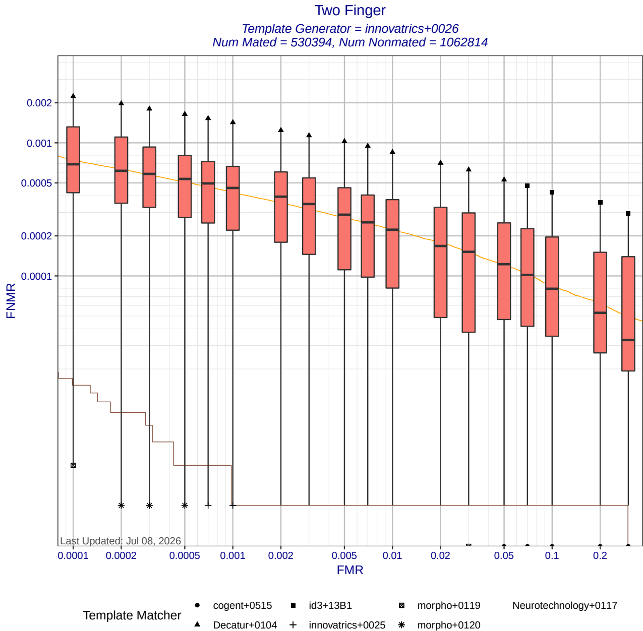
Figure 6: Two Finger DET statistics for template generator innovatrics+0026. Each box shows the distribution of FNRs at a fixed FMR across different matchers. The whisker ends show the minimum and maximum FNRs. The brown curve shows the DET curve when the matcher and template generators were submitted by the same participant. The orange DET curve shows pooled performance when all matchers use templates created by innovatrics+0026. Score-level fusion is achieved by averaging the scores for left and right index fingers.
