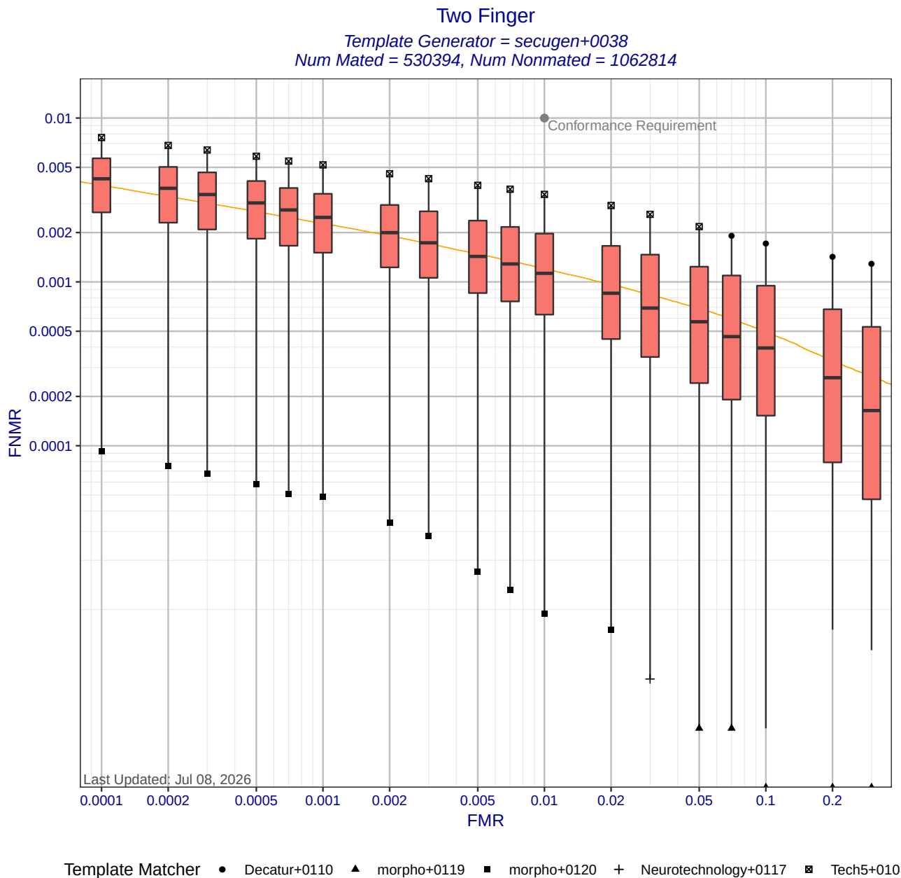
Figure 6: Two Finger DET statistics for template generator secugen+0038. Each box shows the distribution of FNMRs at a fixed FMR across different matchers. The whisker ends show the minimum and maximum FNMRs. The orange DET curve shows pooled performance when all matchers use templates created by secugen+0038. Score-level fusion is achieved by averaging the scores for left and right index fingers.
