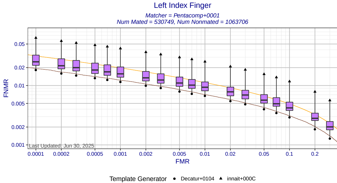
Figure 4: Left index finger DET statistics for matcher Pentacomp+0001. Each box shows the distribution of FNMRs at a fixed FMR across all MINEX III compliant template generators. The ends of the whiskers show the minimum and maximum FNMRs. The orange DET curve shows pooled performance against all template generators.
