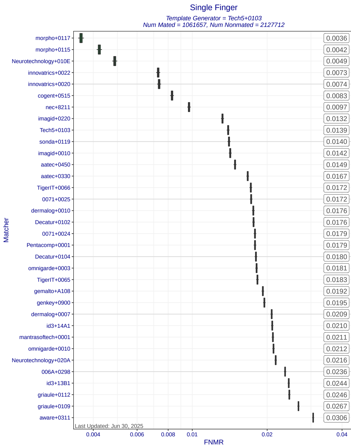
Figure 5: Single Finger FNMNRs at FMR=0.0001 when MINEX III compliant matchers compare templates created by template generator Tech5+0103. Each box represents uncertainty about the true FNMNR. The box edges mark the 50% confidence intervals while the whiskers mark the 90% confidence intervals. The numbers on the right show the actual computed FNMNRs.
