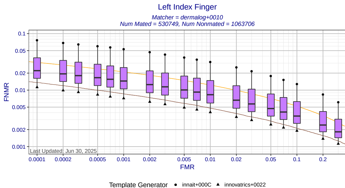
Figure 4: Left index finger DET statistics for matcher dermalog+0010. Each box shows the distribution of FNRs at a fixed FMR across all MINEX III compliant template generators. The ends of whiskers show the minimum and maximum FNRs. The orange DET curve shows pooled performance against all template generators.
