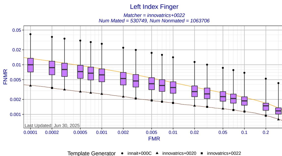
Figure 4: Left index finger DET statistics for matcher innovatrics+0022. Each box shows the distribution of FNMRs at a fixed FMR across all MINEX III compliant template generators. The ends of whiskers show the minimum and maximum FNMRs. The orange DET curve shows pooled performance against all template generators.
