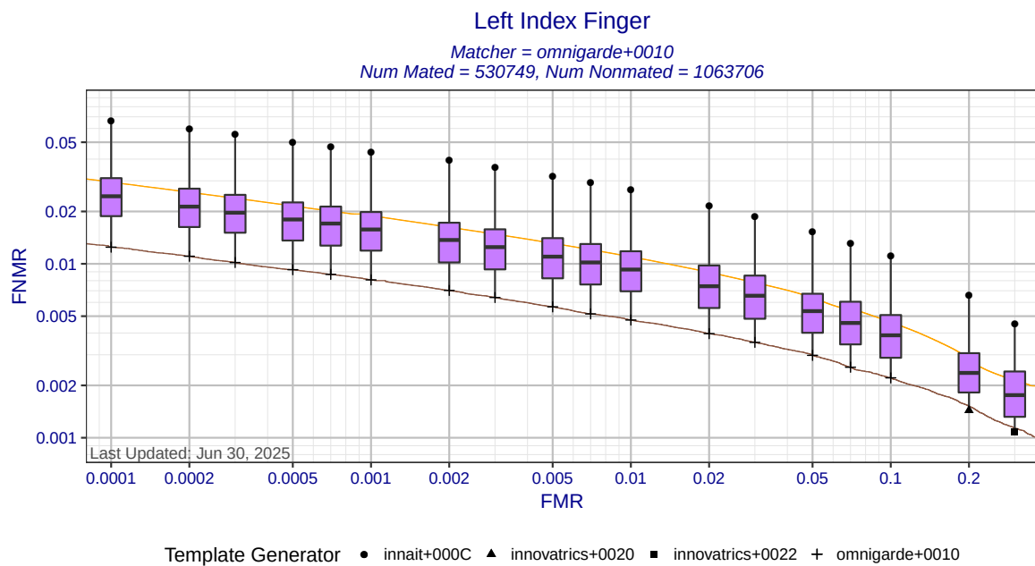
Figure 4: Left index finger DET statistics for matcher omnigarde+0010. Each box shows the distribution of FNRs at a fixed FMR across all MINEX III compliant template generators. The ends of the whiskers show the minimum and maximum FNRs. The orange DET curve shows pooled performance against all template generators.
