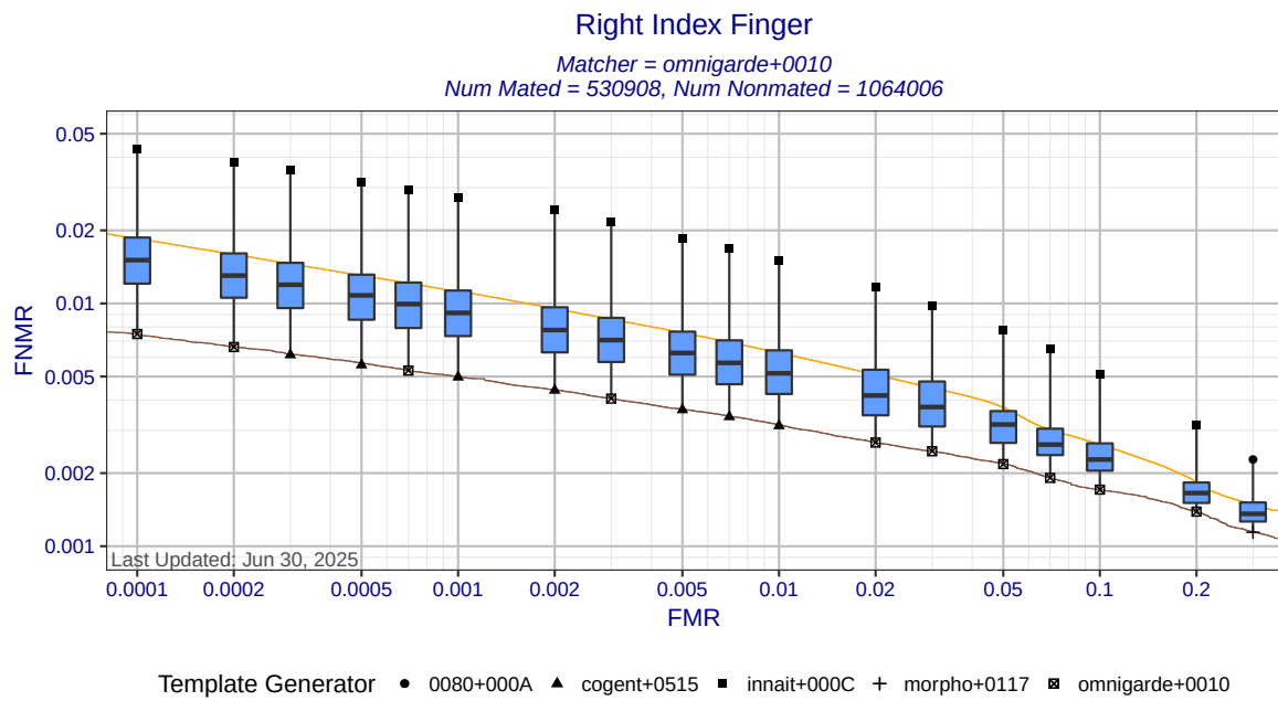
Figure 3: Right index finger DET statistics for matcher omnigarde+0010. Each box shows the distribution of FNRs at a fixed FMR across all MINEX III compliant template generators. The ends of the whiskers show the minimum and maximum FNRs. The orange DET curve shows pooled performance against all template generators.
