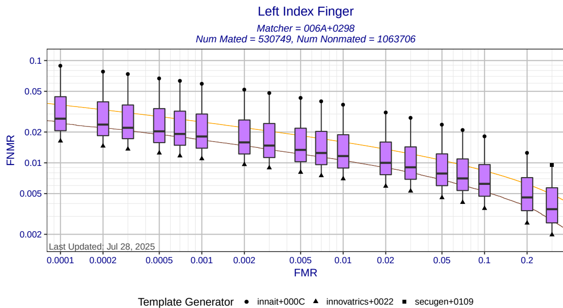
Figure 4: Left index finger DET statistics for matcher 006A+0298. Each box shows the distribution of FNRs at a fixed FMR across all MINEX III compliant template generators. The ends of the whiskers show the minimum and maximum FNRs. The orange DET curve shows pooled performance against all template generators.
