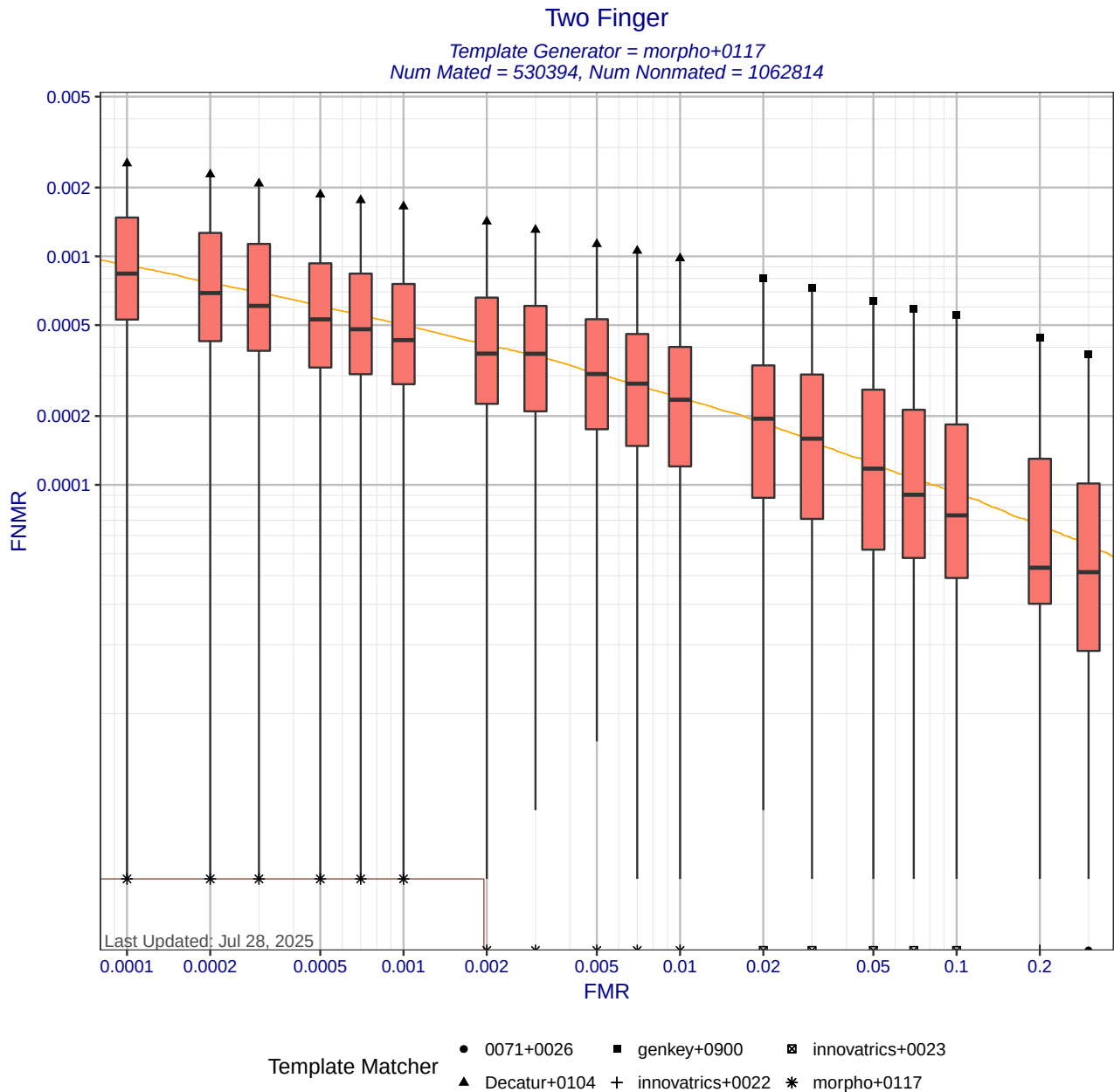
Figure 6: Two Finger DET statistics for template generator morpho+0117. Each box shows the distribution of FNRs at a fixed FMR across different matchers. The whisker ends show the minimum and maximum FNRs. The brown curve shows the DET curve when the matcher and template generators were submitted by the same participant. The orange DET curve shows pooled performance when all matchers use templates created by morpho+0117. Score-level fusion is achieved by averaging the scores for left and right index fingers.
