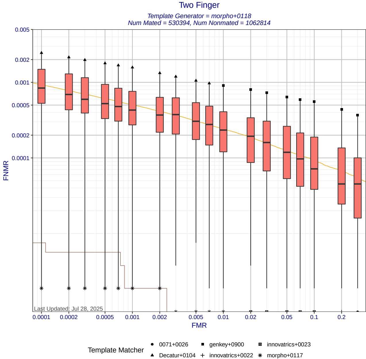
Figure 6: Two Finger DET statistics for template generator morpho+0118. Each box shows the distribution of FNRs at a fixed FMR across different matchers. The whisker ends show the minimum and maximum FNRs. The brown curve shows the DET curve when the matcher and template generators were submitted by the same participant. The orange DET curve shows pooled performance when all matchers use templates created by morpho+0118. Score-level fusion is achieved by averaging the scores for left and right index fingers.
