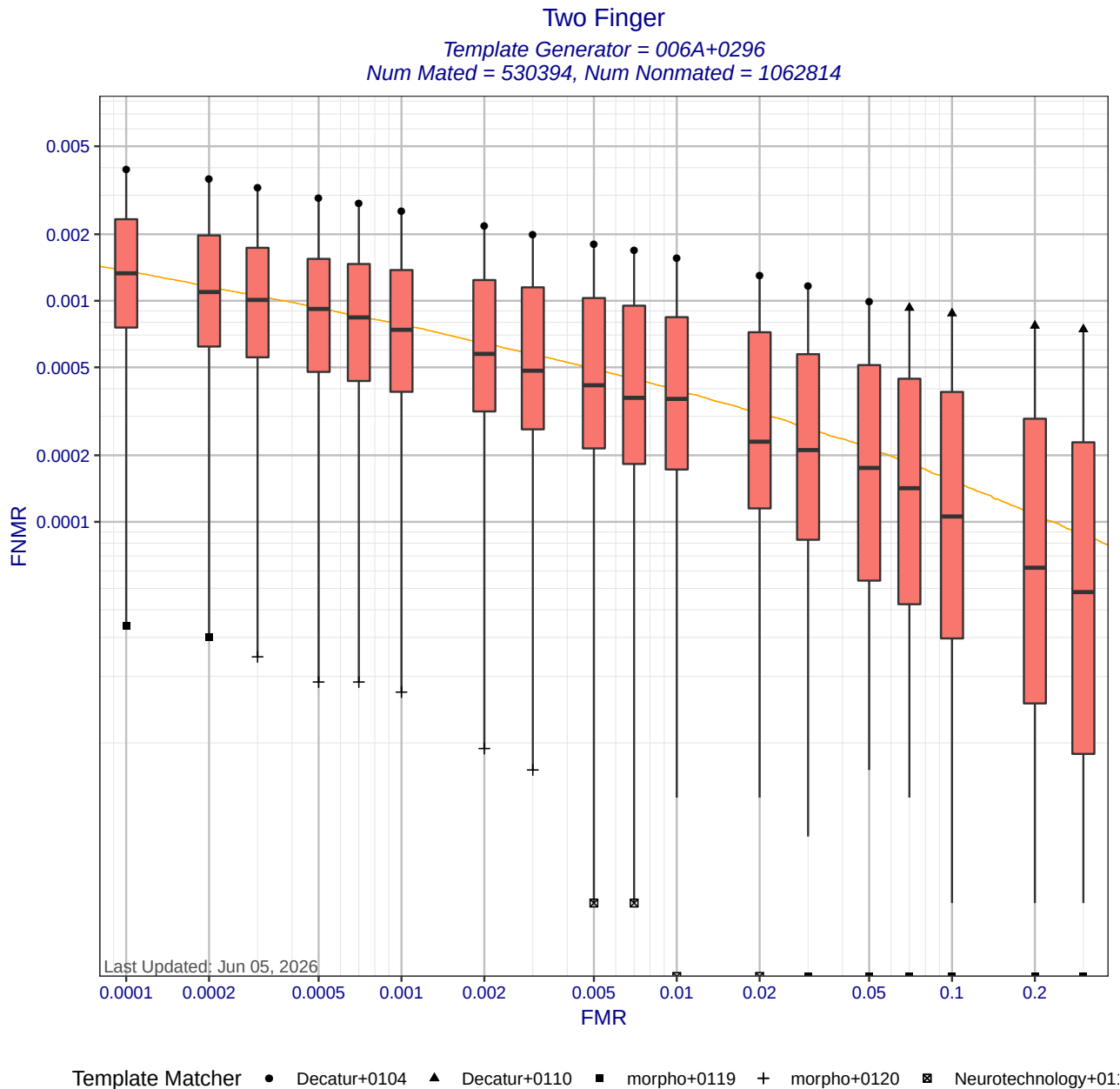
Figure 6: Two Finger DET statistics for template generator 006A+0296. Each box shows the distribution of FNMRs at a fixed FMR across different matchers. The whisker ends show the minimum and maximum FNMRs. The orange DET curve shows pooled performance when all matchers use templates created by 006A+0296. Score-level fusion is achieved by averaging the scores for left and right index fingers.
