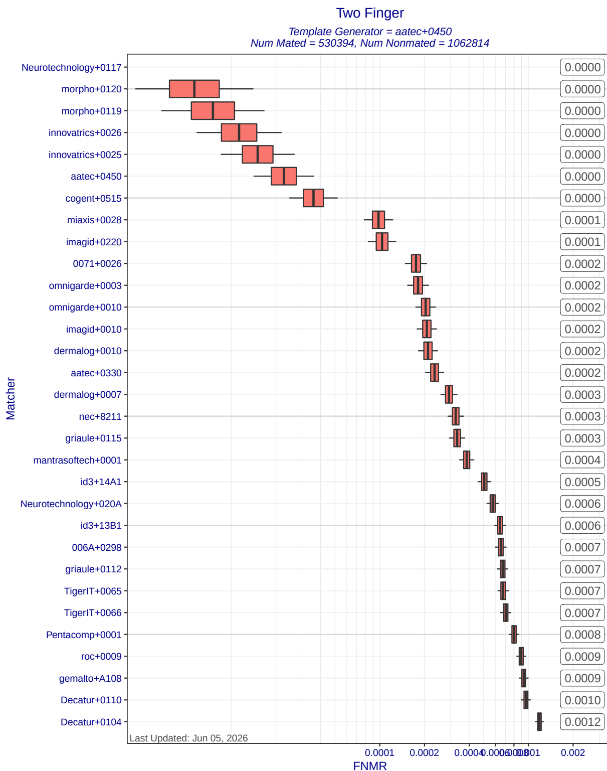
Figure 7: Two Finger FNMR at FMR=0.01 when different matchers compare templates created by template generator aatec+0450. Each box represents uncertainty about the true FNMR. The box edges mark the 50% confidence intervals while the whiskers mark the 90% confidence intervals. The numbers on the right show the actual computed FNMRs. Score-level fusion is achieved by averaging the scores for left and right index fingers.
