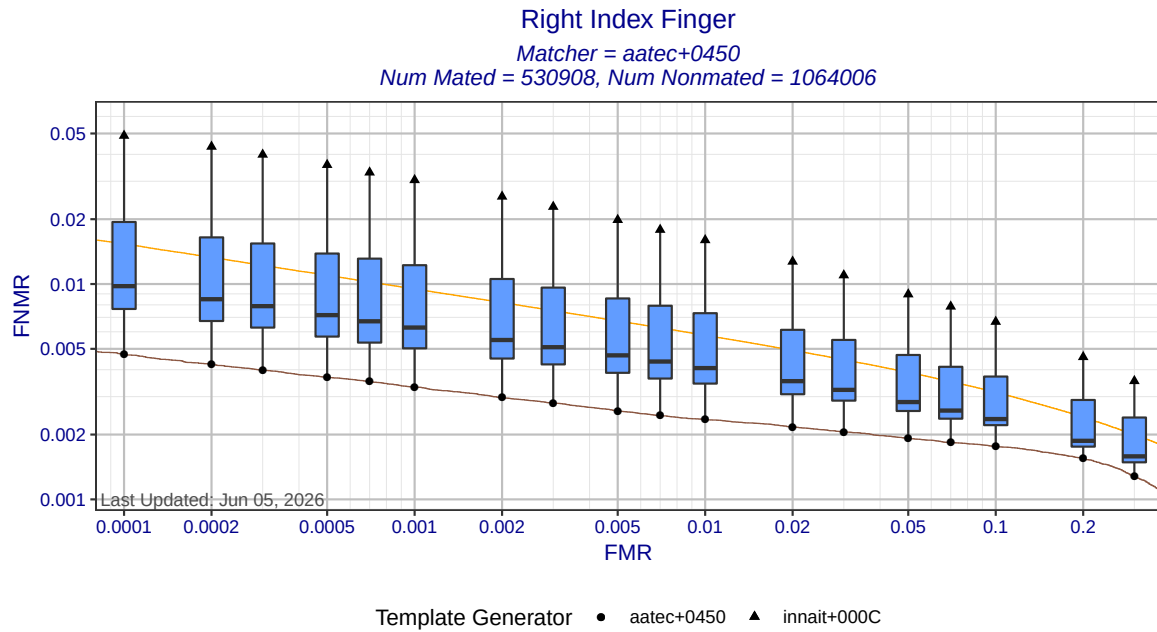
Figure 3: Right index finger DET statistics for matcher aatec+0450. Each box shows the distribution of FNRs at a fixed FMR across all MINEX III compliant template generators. The ends of the whiskers show the minimum and maximum FNRs. The orange DET curve shows pooled performance against all template generators.
