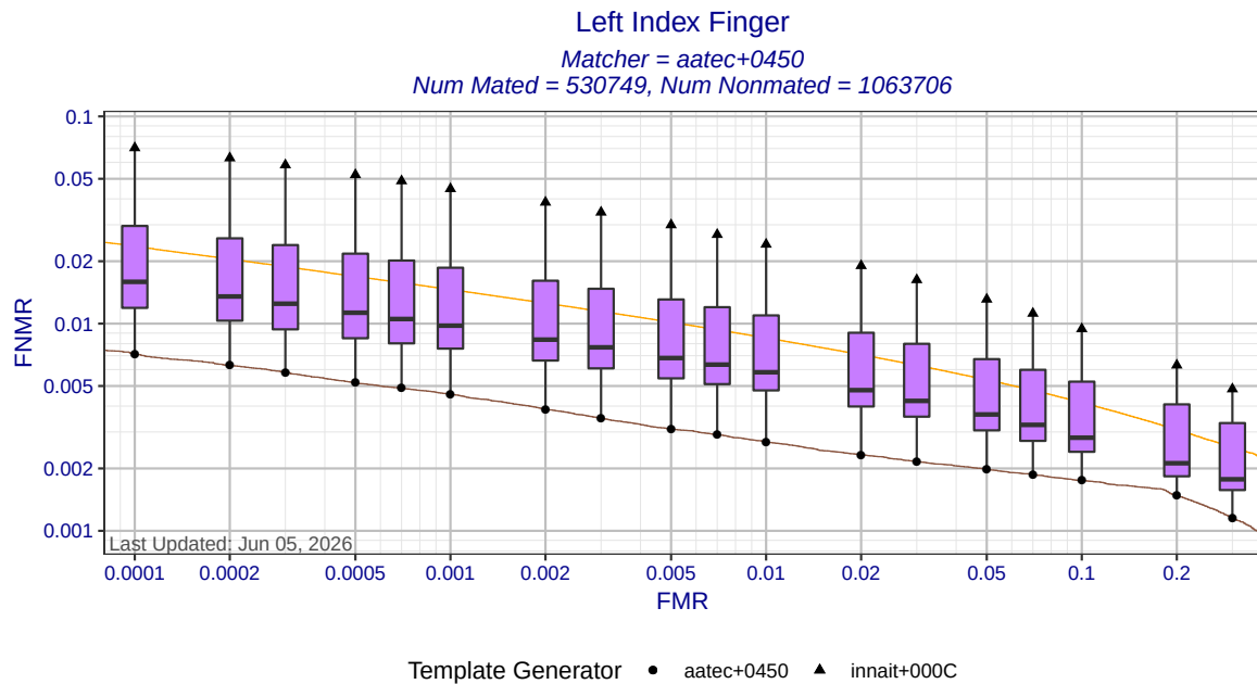
Figure 4: Left index finger DET statistics for matcher aatec+0450. Each box shows the distribution of FNRs at a fixed FMR across all MINEX III compliant template generators. The ends of the whiskers show the minimum and maximum FNRs. The orange DET curve shows pooled performance against all template generators.
