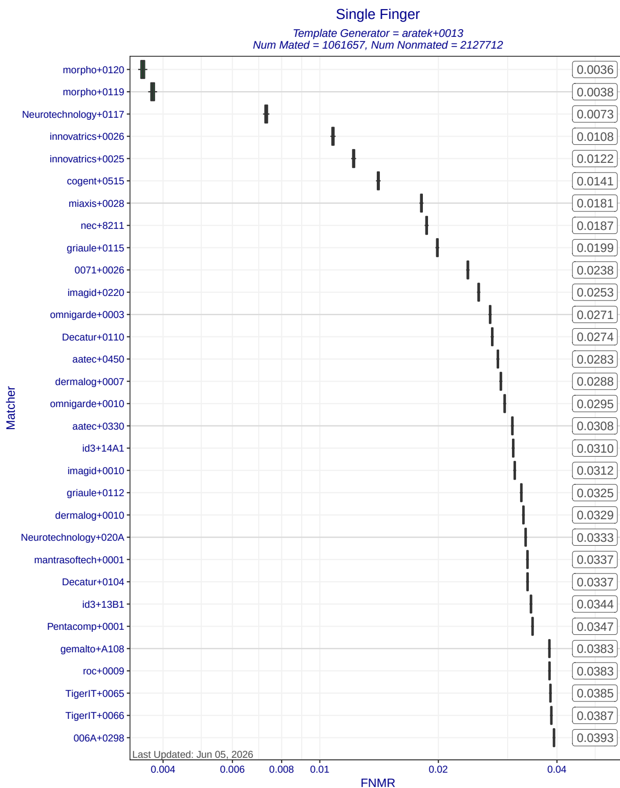
Figure 5: Single Finger FNMNRs at FMR=0.0001 when MINEX III compliant matchers compare templates created by template generator aratek+0013. Each box represents uncertainty about the true FNMNR. The box edges mark the 50% confidence intervals while the whiskers mark the 90% confidence intervals. The numbers on the right show the actual computed FNMNRs.
