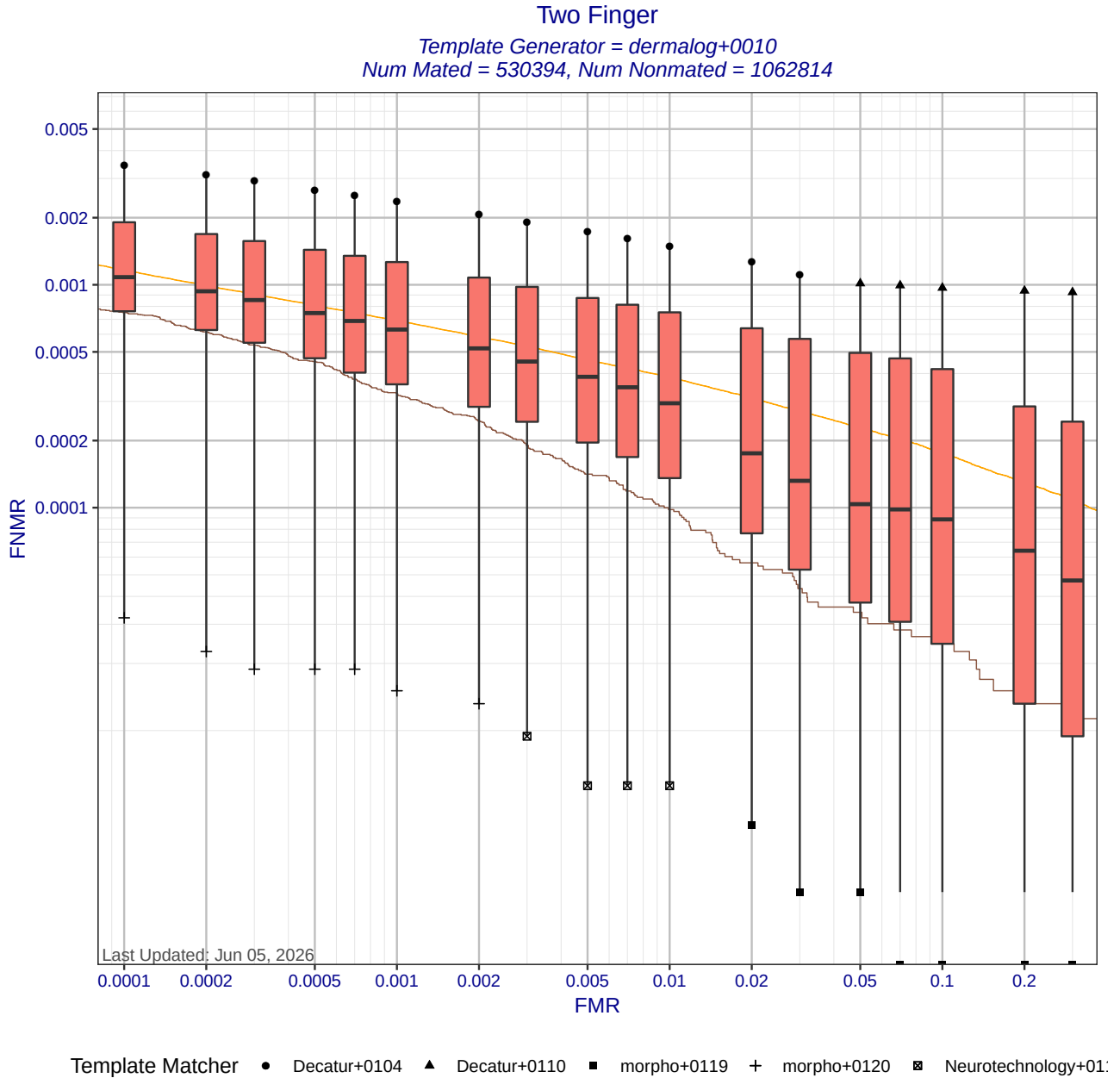
Figure 6: Two Finger DET statistics for template generator dermalog+0010. Each box shows the distribution of FNMIRs at a fixed FMR across different matchers. The whisker ends show the minimum and maximum FNMIRs. The brown curve shows the DET curve when the matcher and template generators were submitted by the same participant. The orange DET curve shows pooled performance when all matchers use templates created by dermalog+0010. Score-level fusion is achieved by averaging the scores for left and right index fingers.
