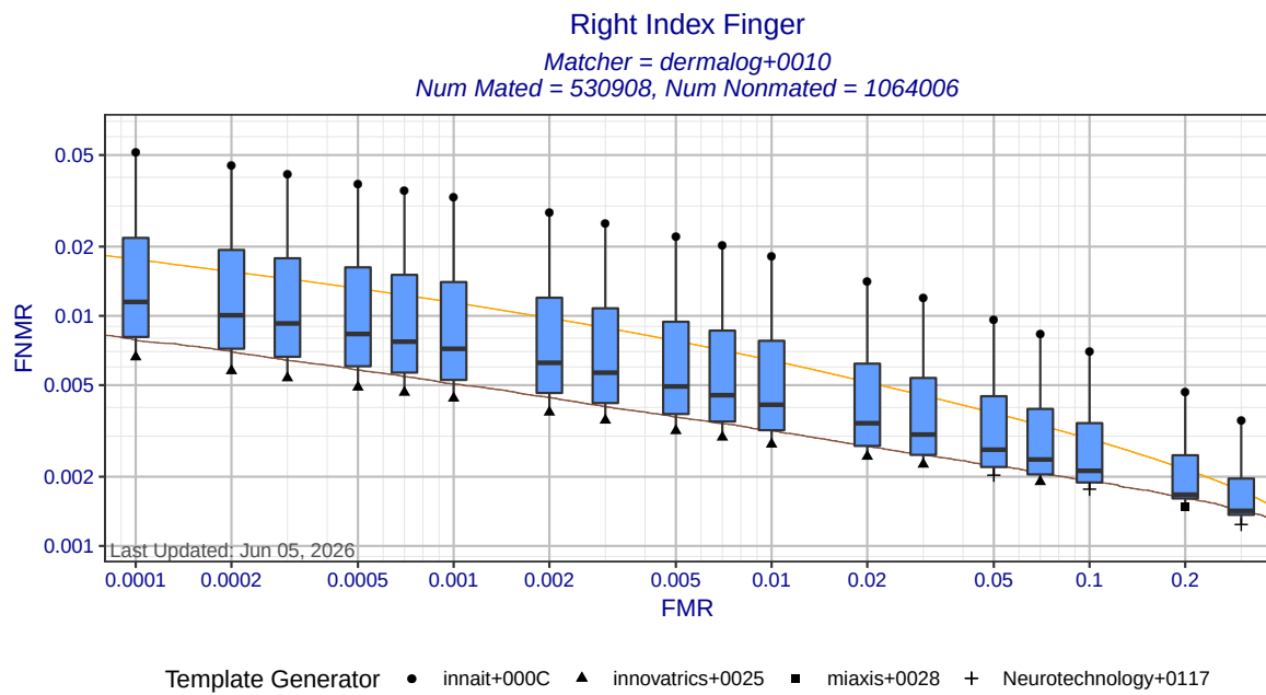
Figure 3: Right index finger DET statistics for matcher dermalog+0010. Each box shows the distribution of FNR at a fixed FMR across all MINEX III compliant template generators. The ends of the whiskers show the minimum and maximum FNRs. The orange DET curve shows pooled performance against all template generators.
