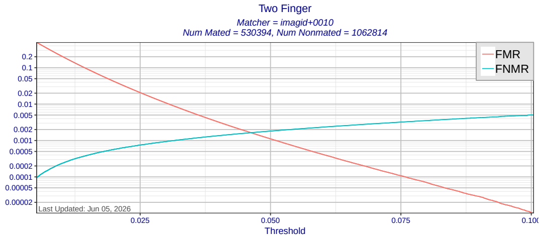
Figure 12: Two finger FMR and FNMR as a function of score threshold for matcher imagid+0010 using templates created by all MINEX III compliant template generators. Score-level fusion is achieved by averaging scores for the left and right index fingers.
