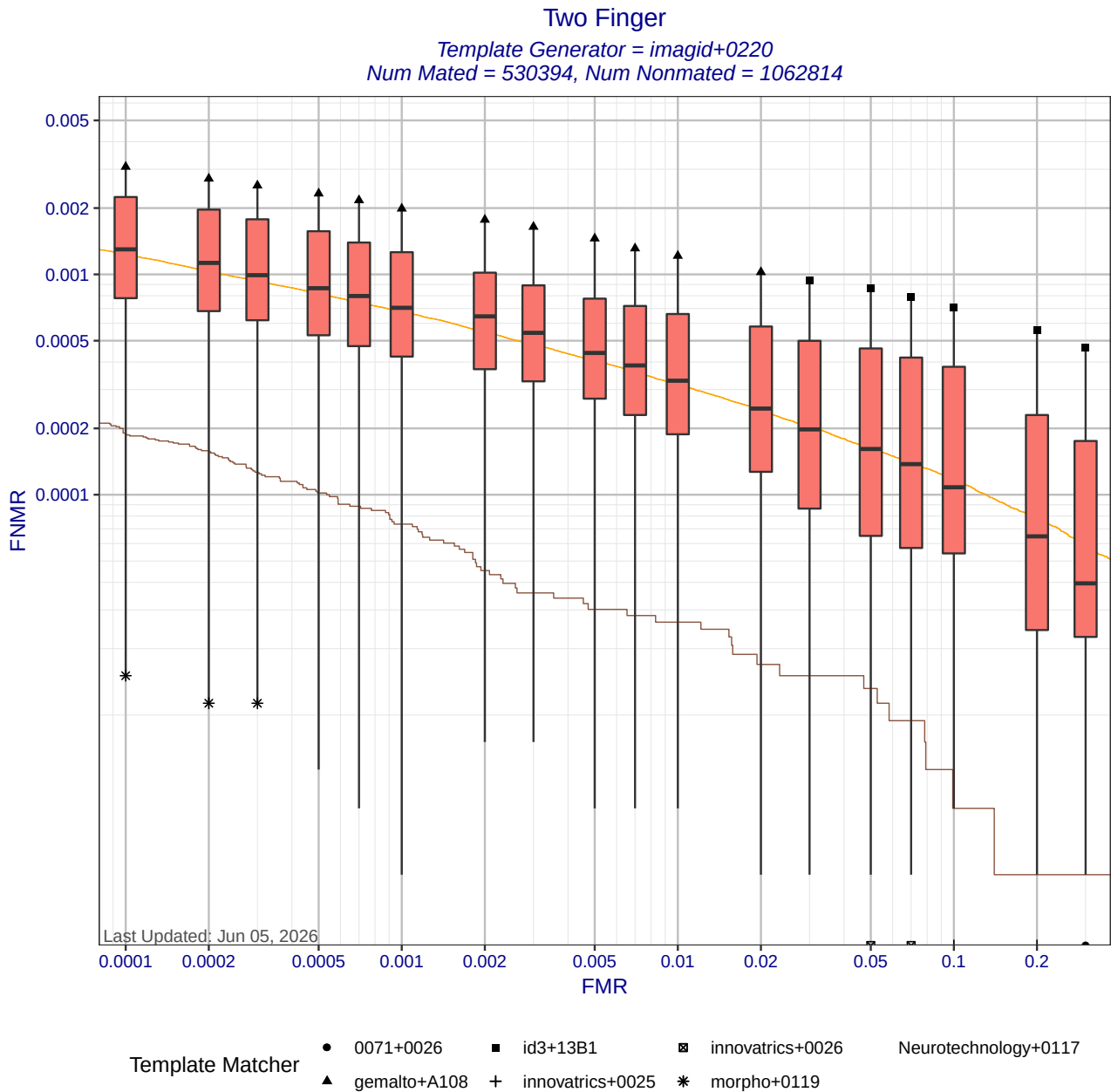
Figure 6: Two Finger DET statistics for template generator imagid+0220. Each box shows the distribution of FNMNRs at a fixed FMR across different matchers. The whisker ends show the minimum and maximum FNMNRs. The brown curve shows the DET curve when the matcher and template generators were submitted by the same participant. The orange DET curve shows pooled performance when all matchers use templates created by imagid+0220. Score-level fusion is achieved by averaging the scores for left and right index fingers.
