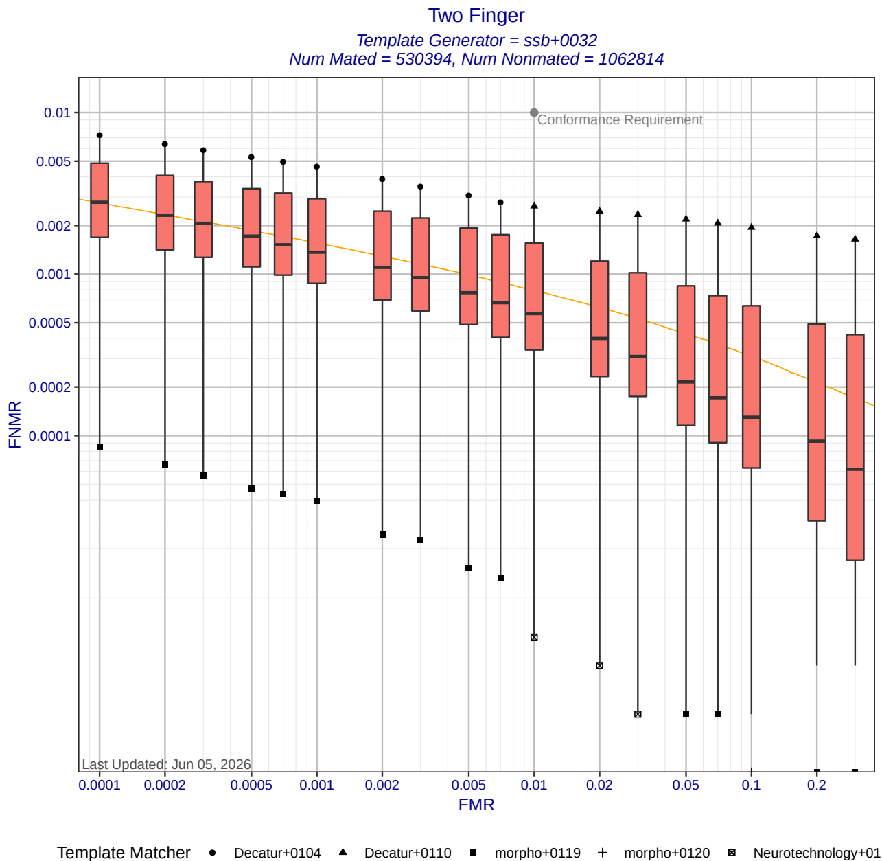
Figure 6: Two Finger DET statistics for template generator ssb+0032. Each box shows the distribution of FNMNRs at a fixed FMR across different matchers. The whisker ends show the minimum and maximum FNMNRs. The orange DET curve shows pooled performance when all matchers use templates created by ssb+0032. Score-level fusion is achieved by averaging the scores for left and right index fingers.
