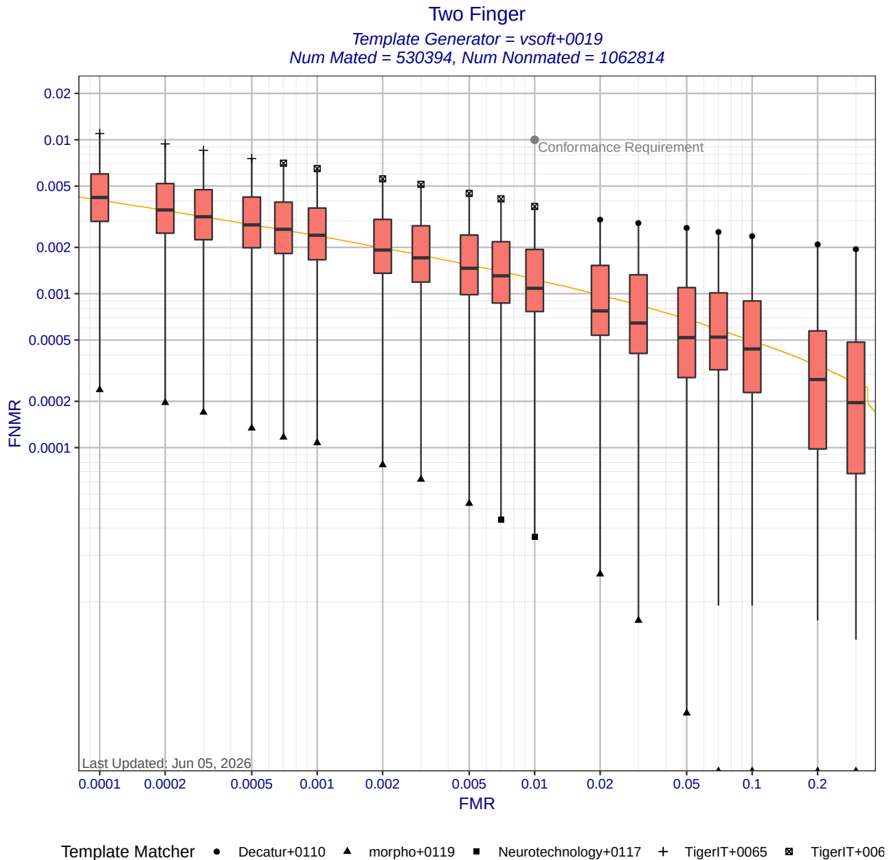
Figure 6: Two Finger DET statistics for template generator vsoft+0019. Each box shows the distribution of FNRs at a fixed FMR across different matchers. The whisker ends show the minimum and maximum FNRs. The orange DET curve shows pooled performance when all matchers use templates created by vsoft+0019. Score-level fusion is achieved by averaging the scores for left and right index fingers.
