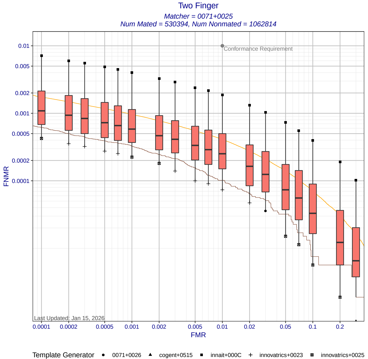
Figure 7: Two finger DET statistics for matcher 0071+0025. Each box shows the distribution of FNMRs at a fixed FMR across all MINEX III compliant template generators. The whisker ends show the minimum and maximum FNMRs. The orange DET curve shows pooled performance against all template generators. Score-level fusion is achieved by averaging the scores for left and right index fingers.
