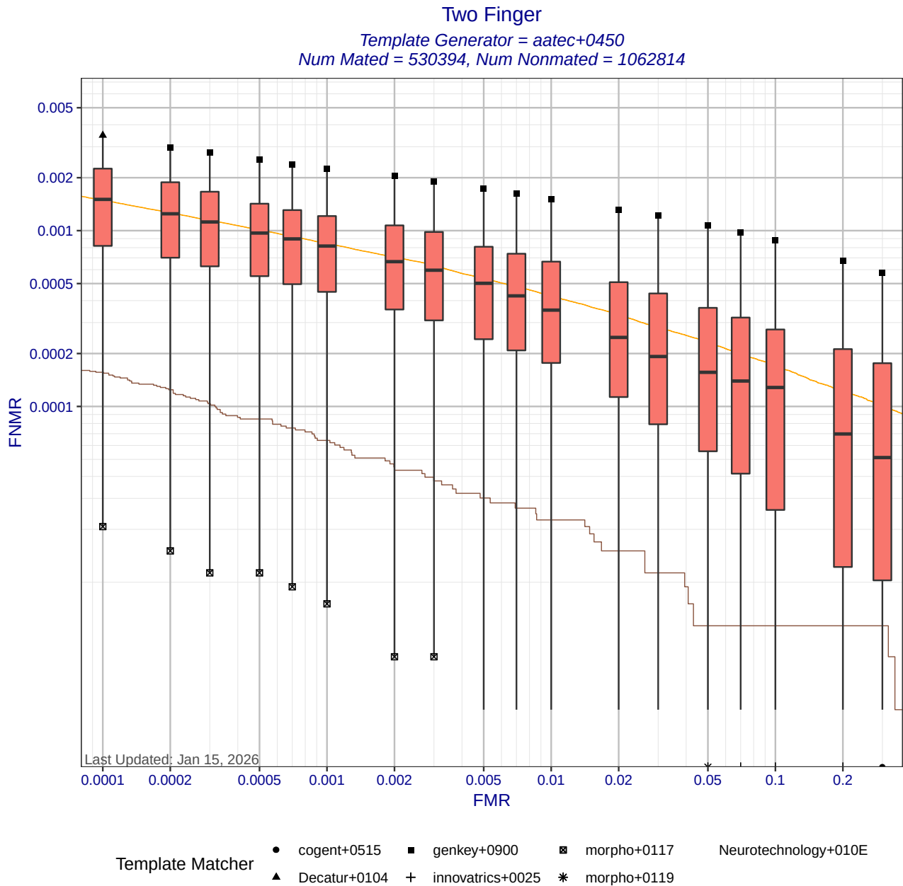
Figure 6: Two Finger DET statistics for template generator aatec+0450. Each box shows the distribution of FNMNRs at a fixed FMR across different matchers. The whisker ends show the minimum and maximum FNMNRs. The brown curve shows the DET curve when the matcher and template generators were submitted by the same participant. The orange DET curve shows pooled performance when all matchers use templates created by aatec+0450. Score-level fusion is achieved by averaging the scores for left and right index fingers.
