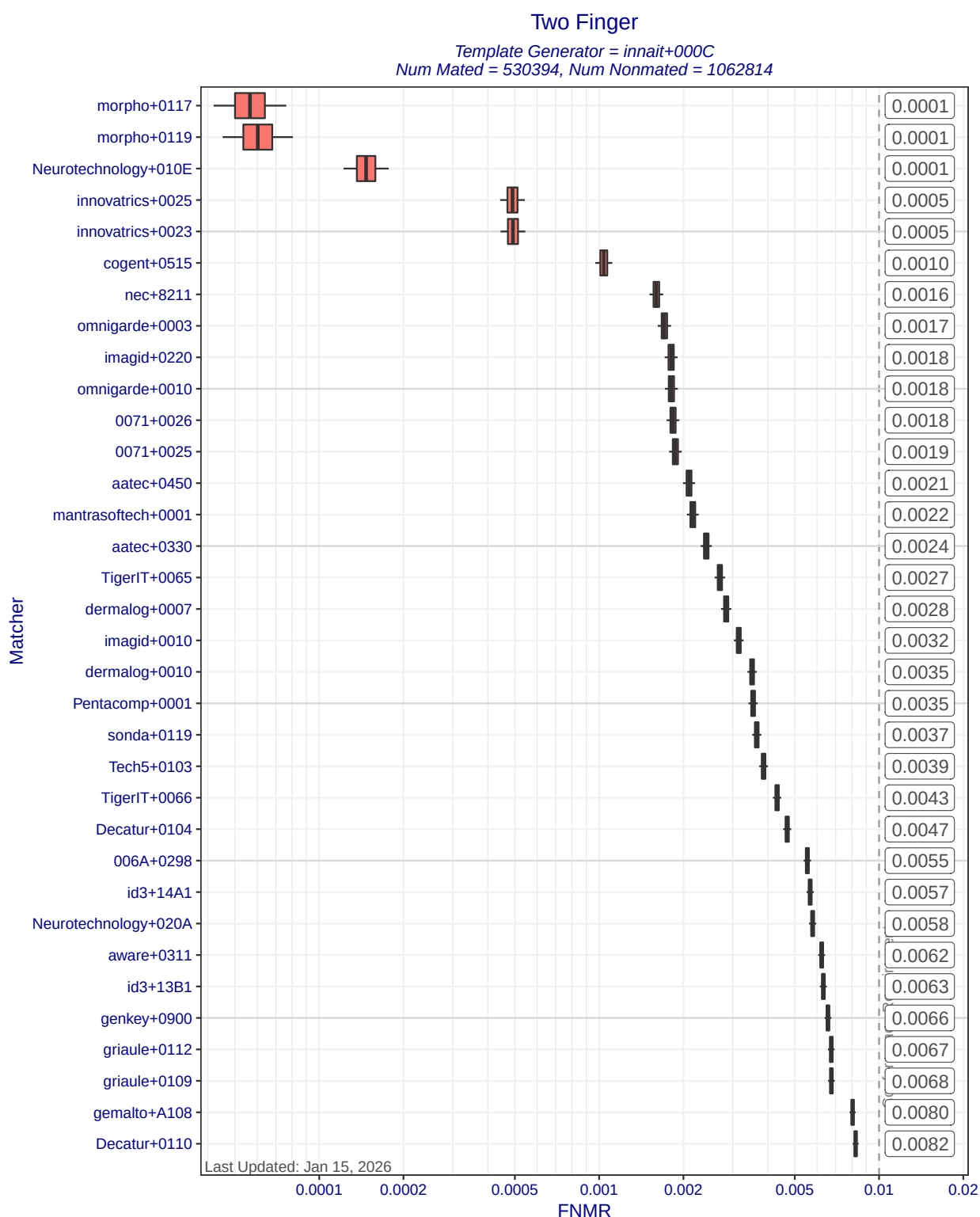
Figure 7: Two Finger FNMR at FMR=0.01 when different matchers compare templates created by template generator innait+000C. Each box represents uncertainty about the true FNMR. The box edges mark the 50% confidence intervals while the whiskers mark the 90% confidence intervals. The numbers on the right show the actual computed FNMRs. Score-level fusion is achieved by averaging the scores for left and right index fingers.
