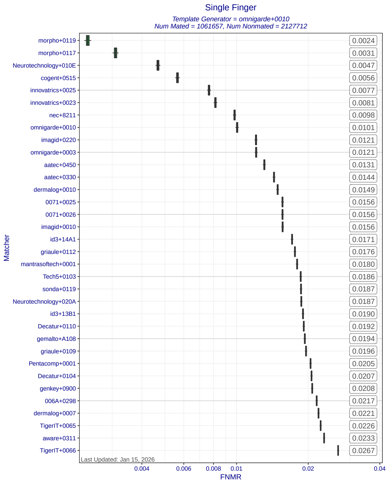
Figure 5: Single Finger FNMRs at FMR=0.0001 when MINEX III compliant matchers compare templates created by template generator omnigarde+0010. Each box represents uncertainty about the true FNMR. The box edges mark the 50% confidence intervals while the whiskers mark the 90% confidence intervals. The numbers on the right show the actual computed FNMRs.
