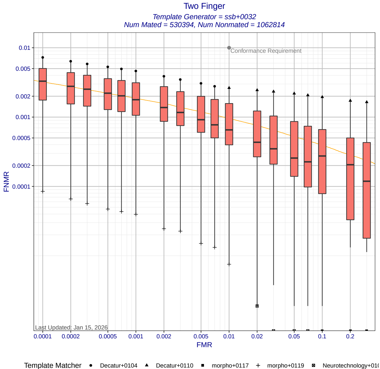
Figure 6: Two Finger DET statistics for template generator ssb+0032. Each box shows the distribution of FNMRs at a fixed FMR across different matchers. The whisker ends show the minimum and maximum FNMRs. The orange DET curve shows pooled performance when all matchers use templates created by ssb+0032. Score-level fusion is achieved by averaging the scores for left and right index fingers.
