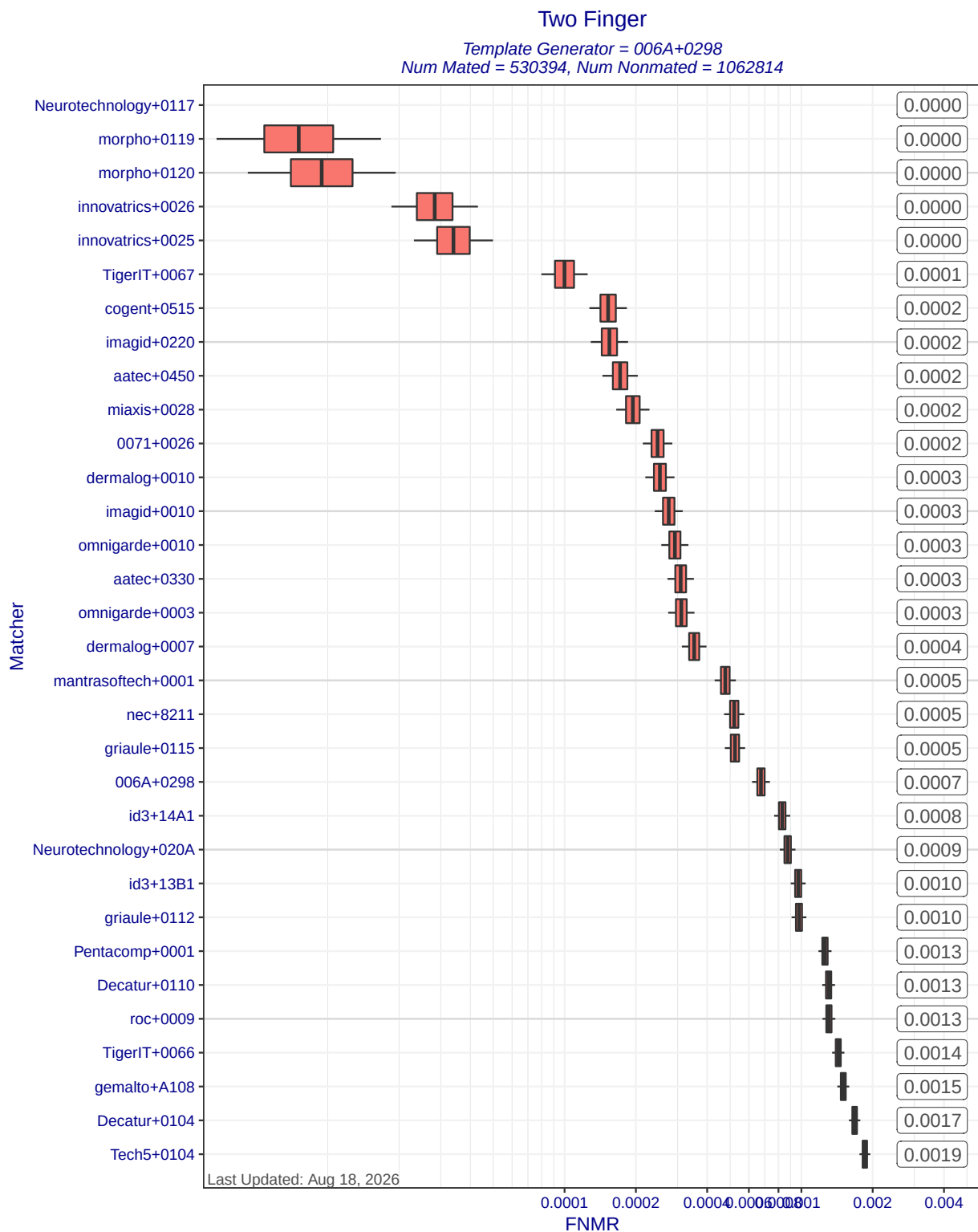
Figure 7: Two Finger FNMR at FMR=0.01 when different matchers compare templates created by template generator 006A+0298. Each box represents uncertainty about the true FNMR. The box edges mark the 50% confidence intervals while the whiskers mark the 90% confidence intervals. The numbers on the right show the actual computed FNMRs. Score-level fusion is achieved by averaging the scores for left and right index fingers.
