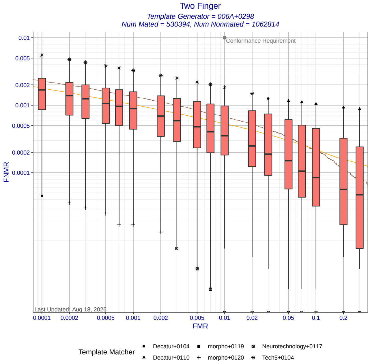
Figure 6: Two Finger DET statistics for template generator 006A+0298. Each box shows the distribution of FNRs at a fixed FMR across different matchers. The whisker ends show the minimum and maximum FNRs. The brown curve shows the DET curve when the matcher and template generators were submitted by the same participant. The orange DET curve shows pooled performance when all matchers use templates created by 006A+0298. Score-level fusion is achieved by averaging the scores for left and right index fingers.
