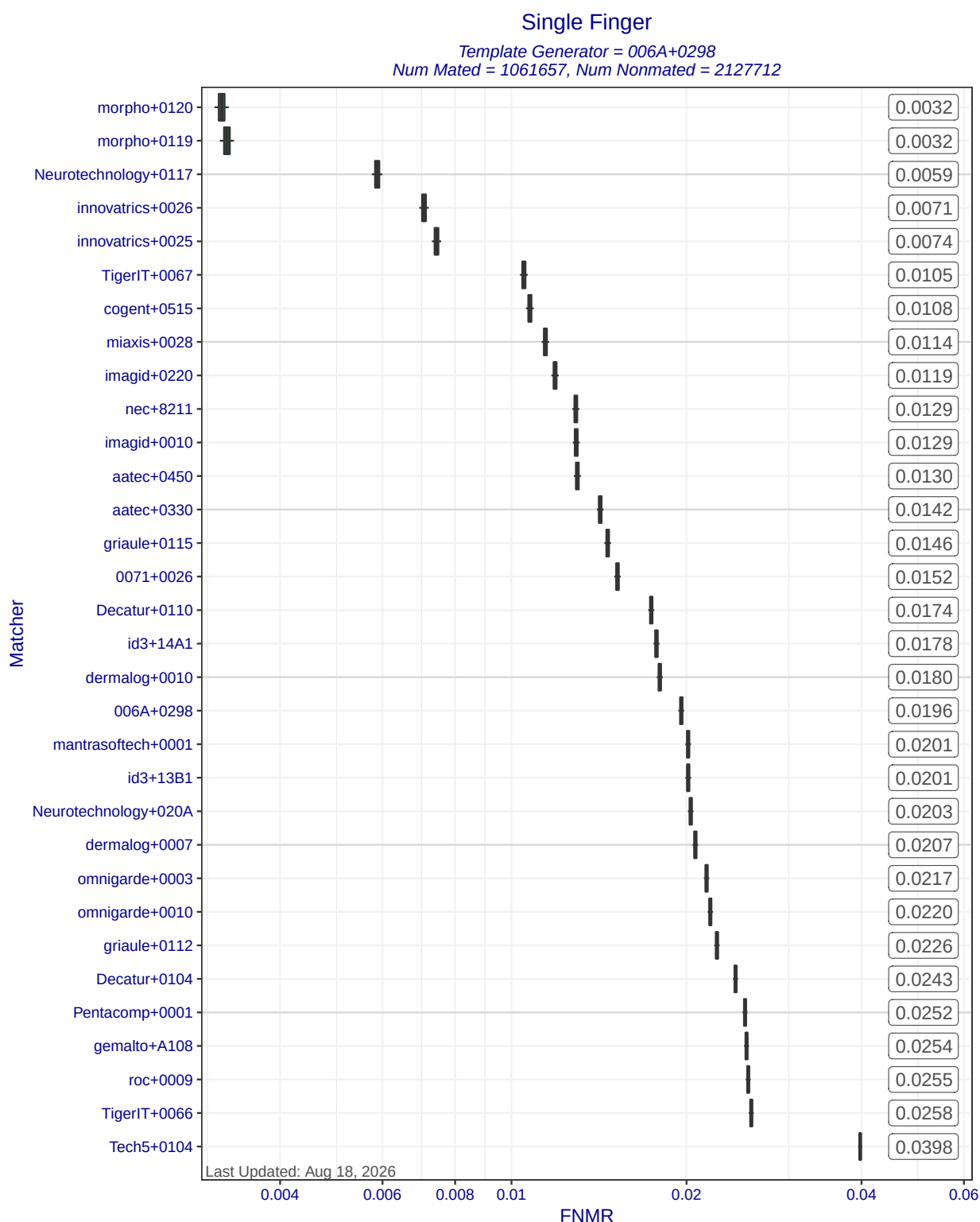
Figure 5: Single Finger FNMRs at FMR=0.0001 when MINEX III compliant matchers compare templates created by template generator 006A+0298. Each box represents uncertainty about the true FNMR. The box edges mark the 50% confidence intervals while the whiskers mark the 90% confidence intervals. The numbers on the right show the actual computed FNMRs.
