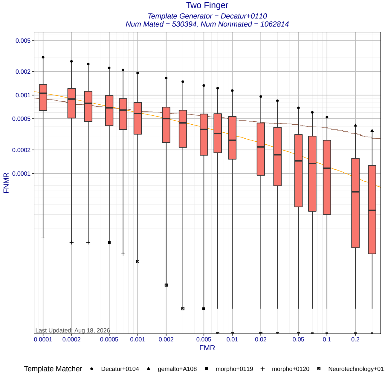
Figure 6: Two Finger DET statistics for template generator Decatur+0110. Each box shows the distribution of FNRs at a fixed FMR across different matchers. The whisker ends show the minimum and maximum FNRs. The brown curve shows the DET curve when the matcher and template generators were submitted by the same participant. The orange DET curve shows pooled performance when all matchers use templates created by Decatur+0110. Score-level fusion is achieved by averaging the scores for left and right index fingers.
