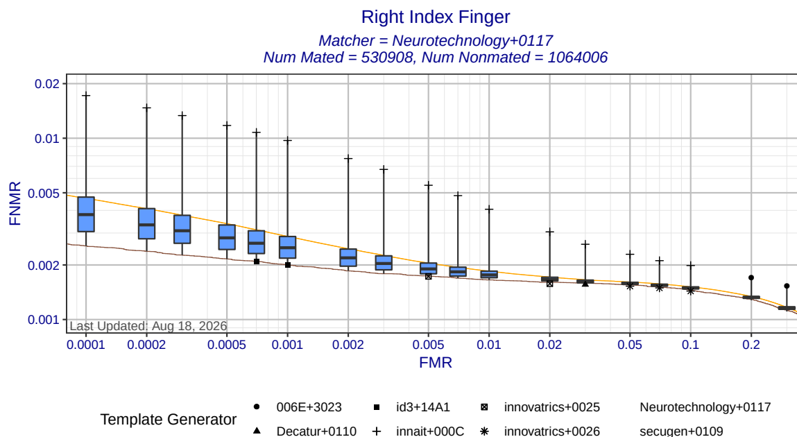
Figure 3: Right index finger DET statistics for matcher Neurotechnology+0117. Each box shows the distribution of FNRs at a fixed FMR across all MINEX III compliant template generators. The ends of the whiskers show the minimum and maximum FNRs. The orange DET curve shows pooled performance against all template generators.
