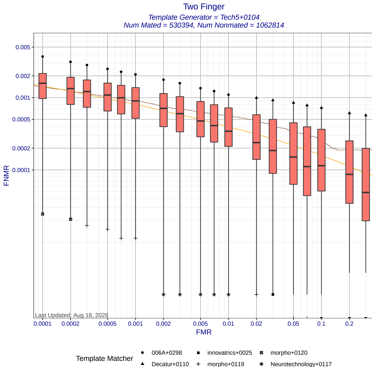
Figure 6: Two Finger DET statistics for template generator Tech5+0104. Each box shows the distribution of FNMIRs at a fixed FMR across different matchers. The whisker ends show the minimum and maximum FNMIRs. The brown curve shows the DET curve when the matcher and template generators were submitted by the same participant. The orange DET curve shows pooled performance when all matchers use templates created by Tech5+0104. Score-level fusion is achieved by averaging the scores for left and right index fingers.
