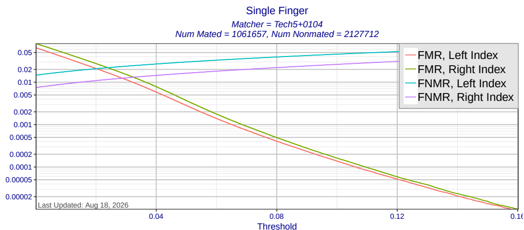
Figure 11: Single finger FMR and FNMR as a function of score threshold for matcher Tech5+0104 using templates created by all MINEX III compliant template generators. Separate curves are presented for left and right index fingers.
