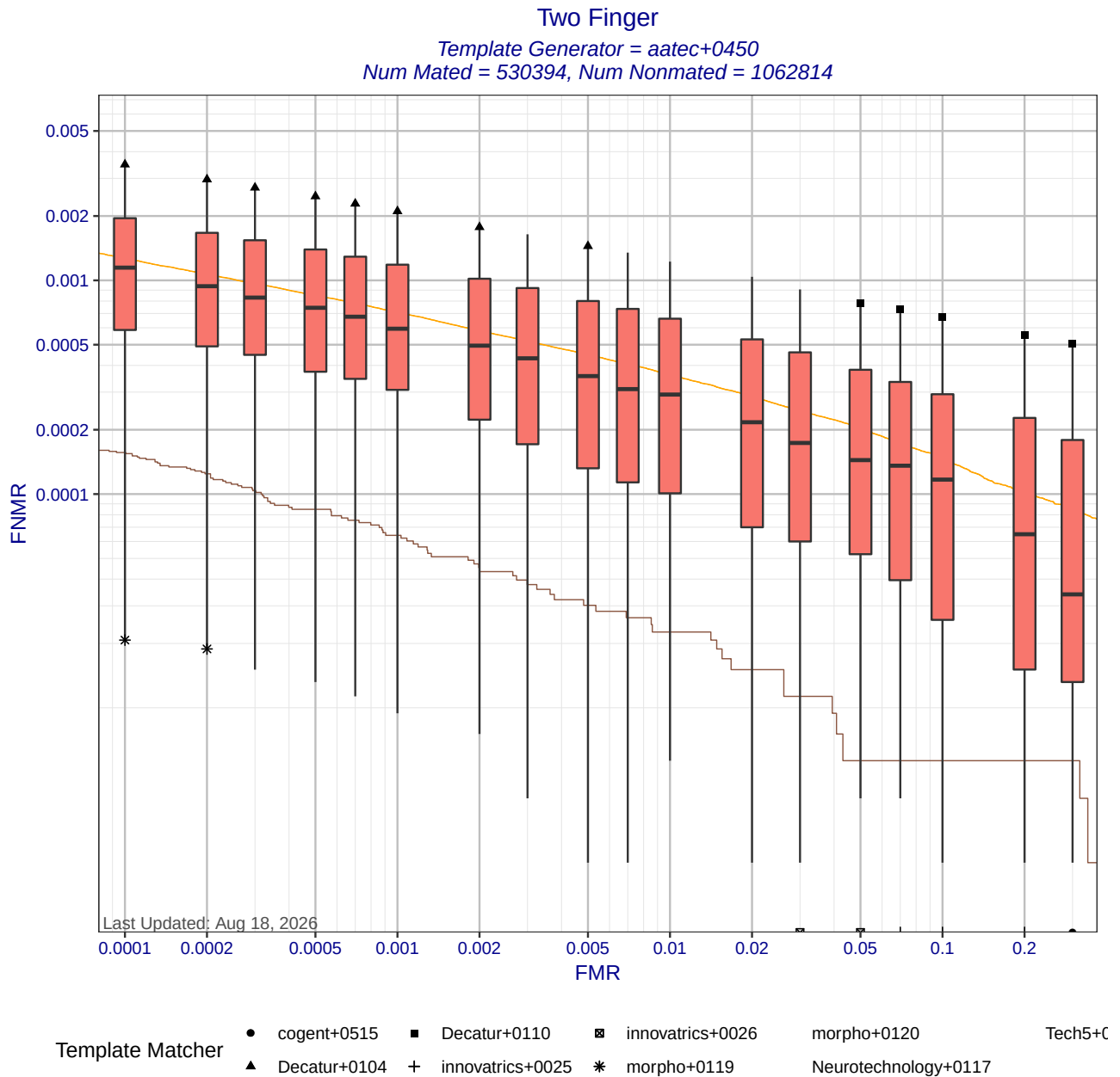
Figure 6: Two Finger DET statistics for template generator aatec+0450. Each box shows the distribution of FNMRs at a fixed FMR across different matchers. The whisker ends show the minimum and maximum FNMRs. The brown curve shows the DET curve when the matcher and template generators were submitted by the same participant. The orange DET curve shows pooled performance when all matchers use templates created by aatec+0450. Score-level fusion is achieved by averaging the scores for left and right index fingers.
