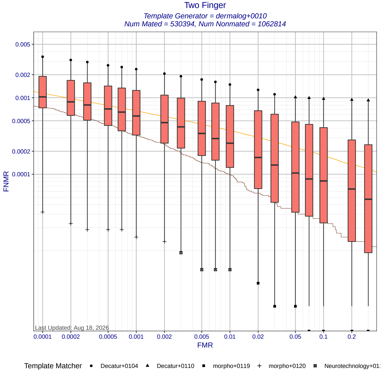
Figure 6: Two Finger DET statistics for template generator dermalog+0010. Each box shows the distribution of FNMRs at a fixed FMR across different matchers. The whisker ends show the minimum and maximum FNMRs. The brown curve shows the DET curve when the matcher and template generators were submitted by the same participant. The orange DET curve shows pooled performance when all matchers use templates created by dermalog+0010. Score-level fusion is achieved by averaging the scores for left and right index fingers.
