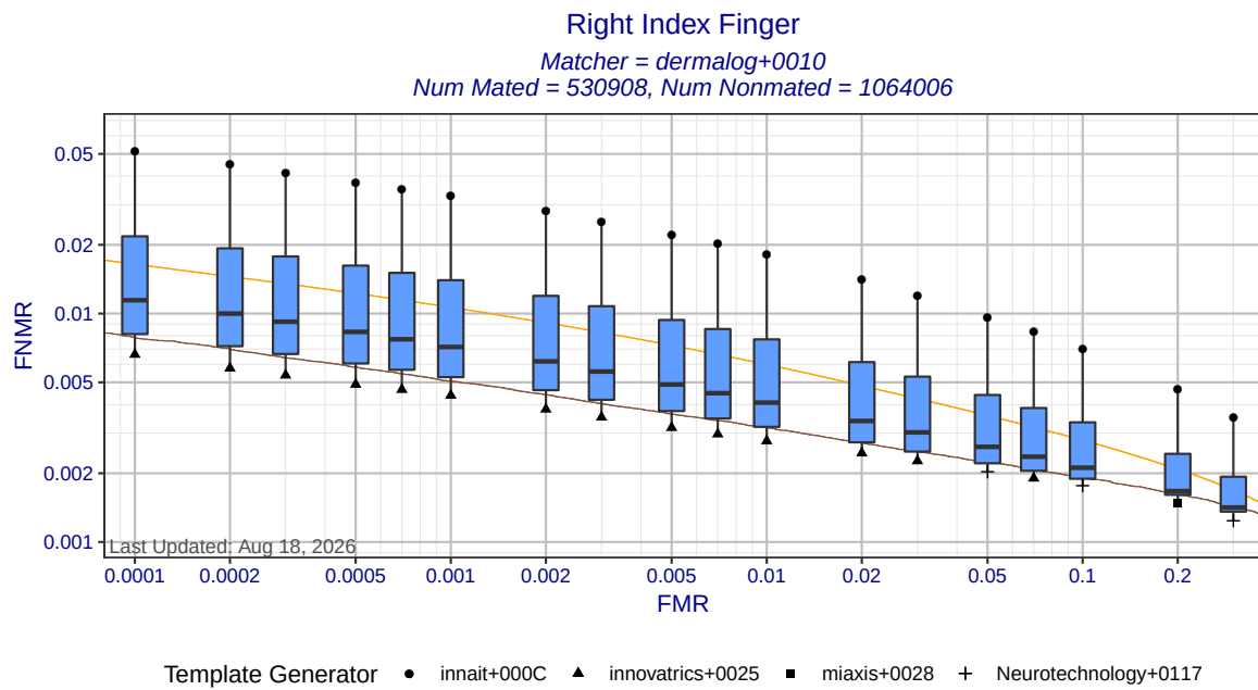
Figure 3: Right index finger DET statistics for matcher dermalog+0010. Each box shows the distribution of FNRs at a fixed FMR across all MINEX III compliant template generators. The ends of the whiskers show the minimum and maximum FNRs. The orange DET curve shows pooled performance against all template generators.
