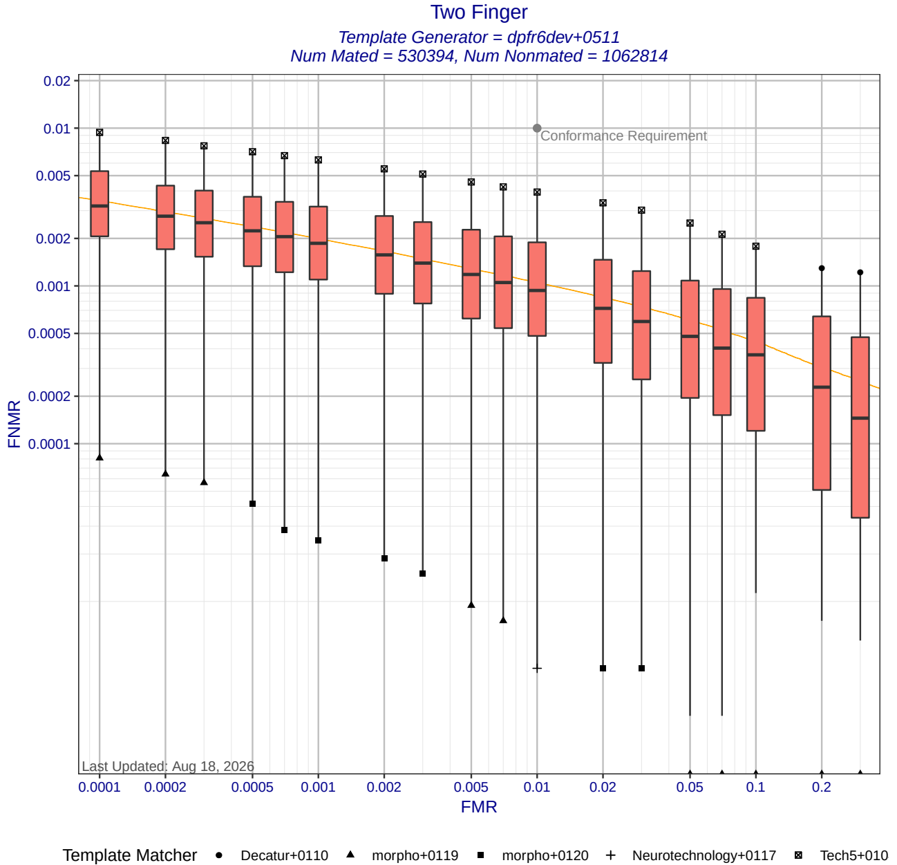
Figure 6: Two Finger DET statistics for template generator dpfr6dev+0511. Each box shows the distribution of FNRs at a fixed FMR across different matchers. The whisker ends show the minimum and maximum FNRs. The orange DET curve shows pooled performance when all matchers use templates created by dpfr6dev+0511. Score-level fusion is achieved by averaging the scores for left and right index fingers.
