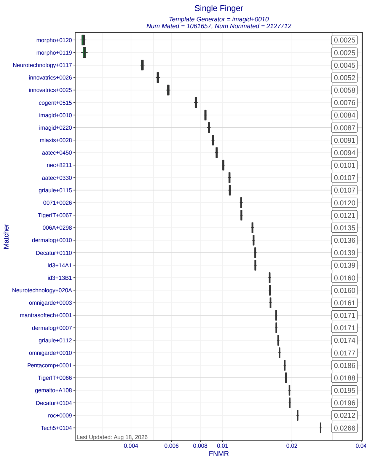
Figure 5: Single Finger FNMRs at FMR=0.0001 when MINEX III compliant matchers compare templates created by template generator imagid+0010. Each box represents uncertainty about the true FNMR. The box edges mark the 50% confidence intervals while the whiskers mark the 90% confidence intervals. The numbers on the right show the actual computed FNMRs.
