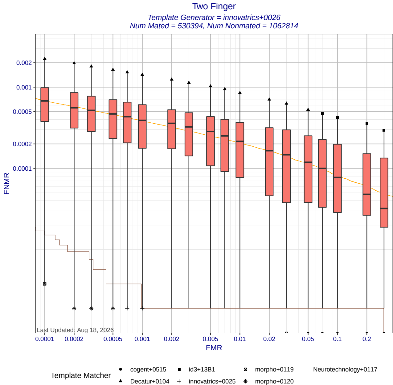
Figure 6: Two Finger DET statistics for template generator innovatrics+0026. Each box shows the distribution of FNMNRs at a fixed FMR across different matchers. The whisker ends show the minimum and maximum FNMNRs. The brown curve shows the DET curve when the matcher and template generators were submitted by the same participant. The orange DET curve shows pooled performance when all matchers use templates created by innovatrics+0026. Score-level fusion is achieved by averaging the scores for left and right index fingers.
