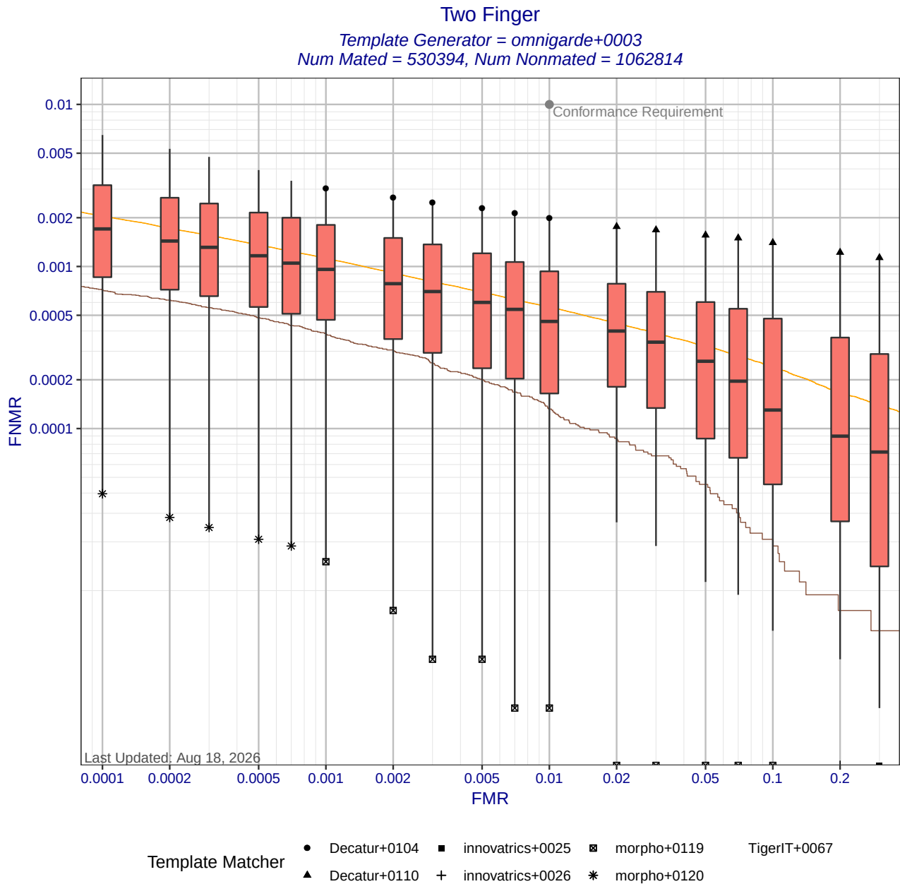
Figure 6: Two Finger DET statistics for template generator omnigarde+0003. Each box shows the distribution of FNMIRs at a fixed FMR across different matchers. The whisker ends show the minimum and maximum FNMIRs. The brown curve shows the DET curve when the matcher and template generators were submitted by the same participant. The orange DET curve shows pooled performance when all matchers use templates created by omnigarde+0003. Score-level fusion is achieved by averaging the scores for left and right index fingers.
