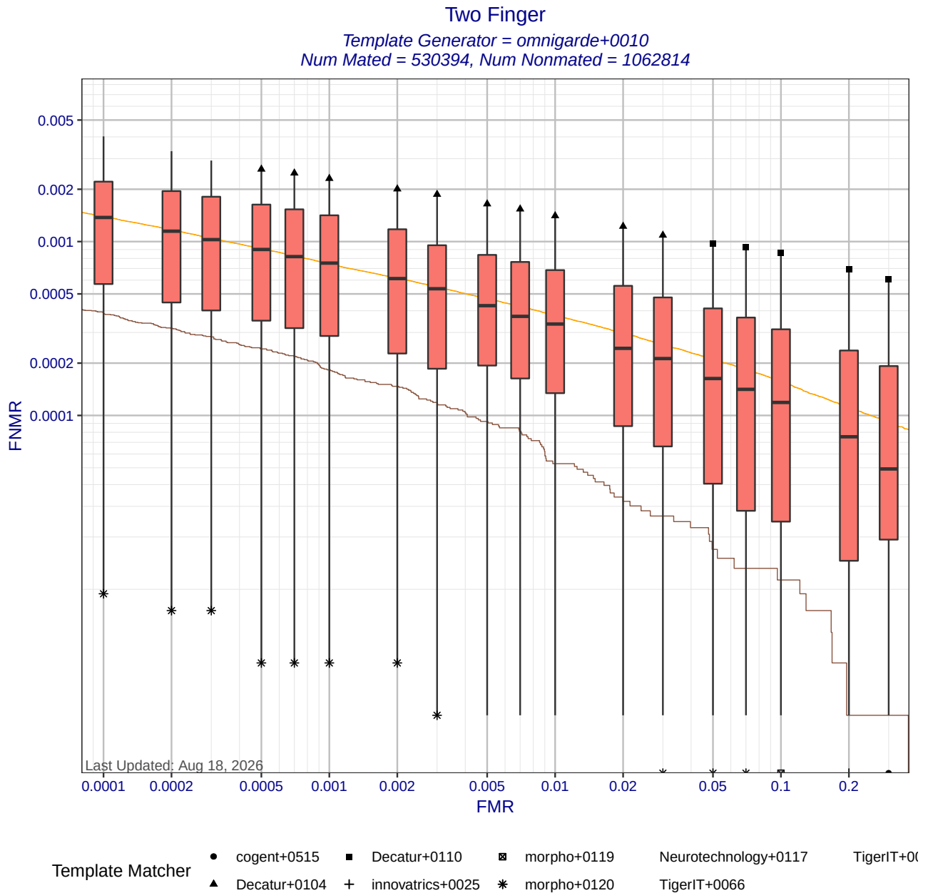
Figure 6: Two Finger DET statistics for template generator omnigarde+0010. Each box shows the distribution of FNMRs at a fixed FMR across different matchers. The whisker ends show the minimum and maximum FNMRs. The brown curve shows the DET curve when the matcher and template generators were submitted by the same participant. The orange DET curve shows pooled performance when all matchers use templates created by omnigarde+0010. Score-level fusion is achieved by averaging the scores for left and right index fingers.
