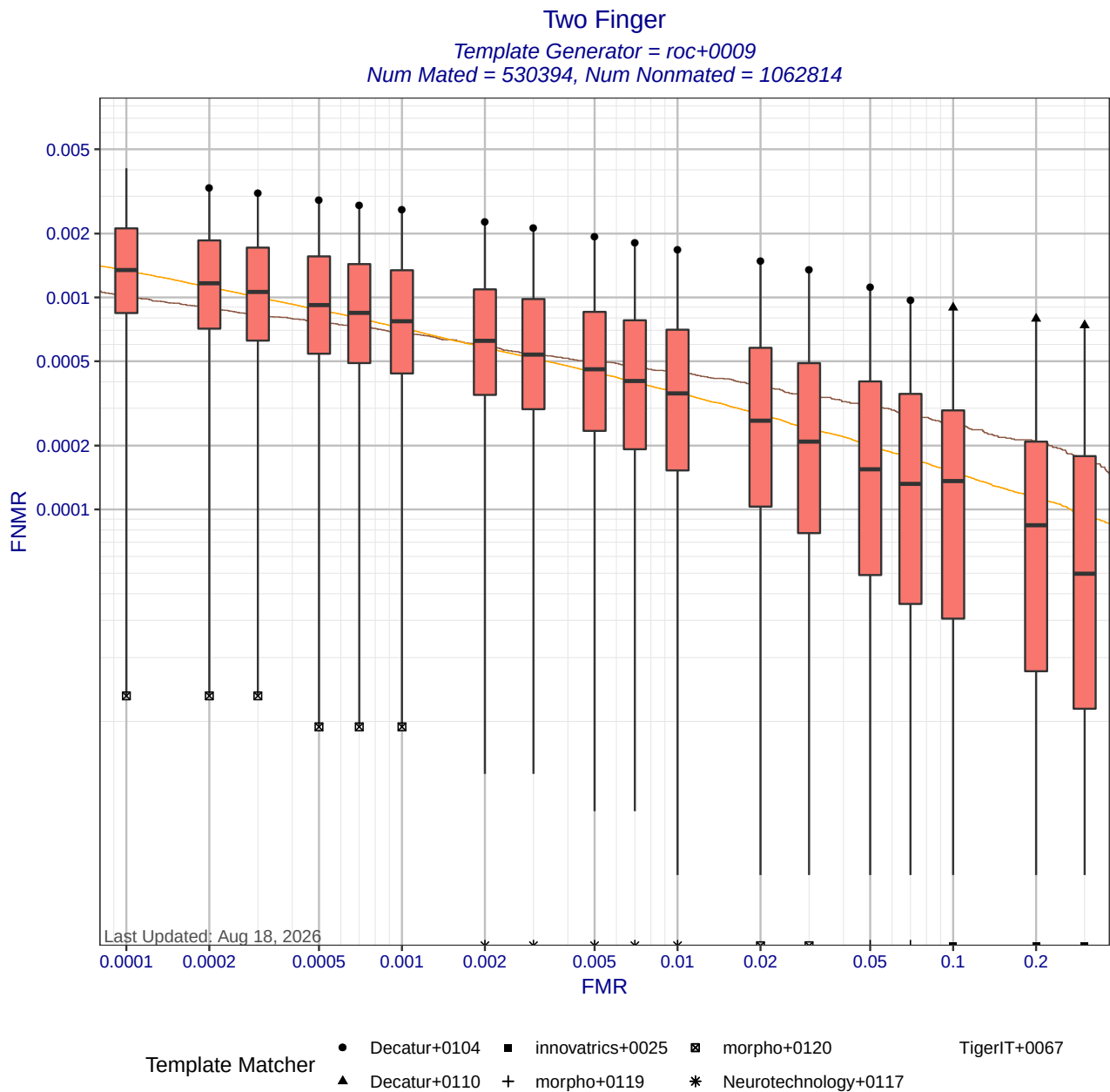
Figure 6: Two Finger DET statistics for template generator roc+0009. Each box shows the distribution of FNMIRs at a fixed FMR across different matchers. The whisker ends show the minimum and maximum FNMIRs. The brown curve shows the DET curve when the matcher and template generators were submitted by the same participant. The orange DET curve shows pooled performance when all matchers use templates created by roc+0009. Score-level fusion is achieved by averaging the scores for left and right index fingers.
