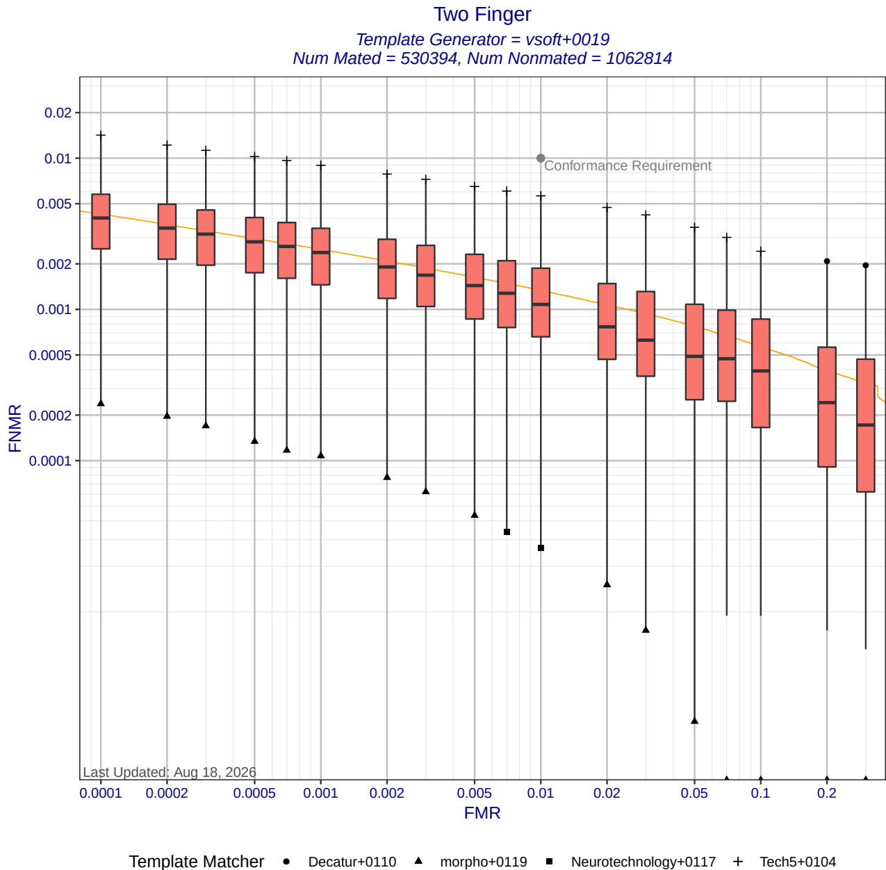
Figure 6: Two Finger DET statistics for template generator vsoft+0019. Each box shows the distribution of FNMRs at a fixed FMR across different matchers. The whisker ends show the minimum and maximum FNMRs. The orange DET curve shows pooled performance when all matchers use templates created by vsoft+0019. Score-level fusion is achieved by averaging the scores for left and right index fingers.
