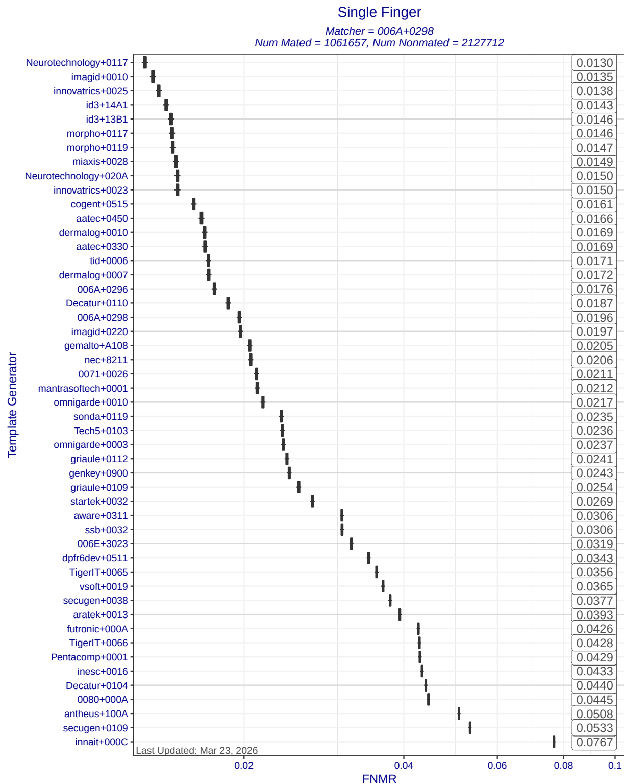
Figure 5: Single finger FNMRs at FMR = 0.0001 when matcher 006A+0298 compares templates created by different template generators. The ends of the whiskers show the minimum and maximum FNMRs. Each box represents uncertainty about the true FNMR. The box edges mark the 50% confidence intervals while the whiskers mark the 90% confidence intervals. The numbers on the right show the actual computed FNMRs.
