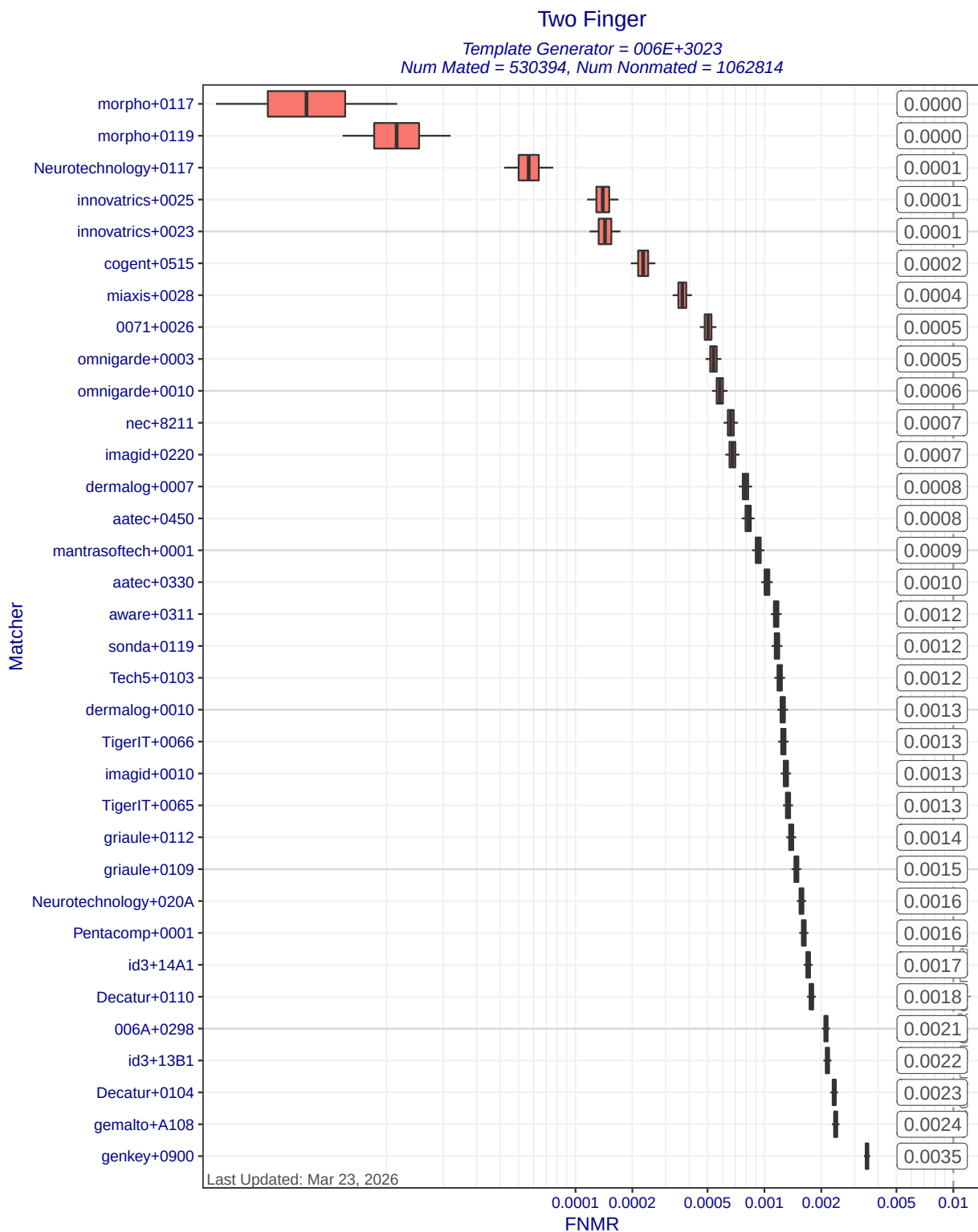
Figure 7: Two Finger FNMR at FMR=0.01 when different matchers compare templates created by template generator 006E+3023. Each box represents uncertainty about the true FNMR. The box edges mark the 50% confidence intervals while the whiskers mark the 90% confidence intervals. The numbers on the right show the actual computed FNMRs. Score-level fusion is achieved by averaging the scores for left and right index fingers.
