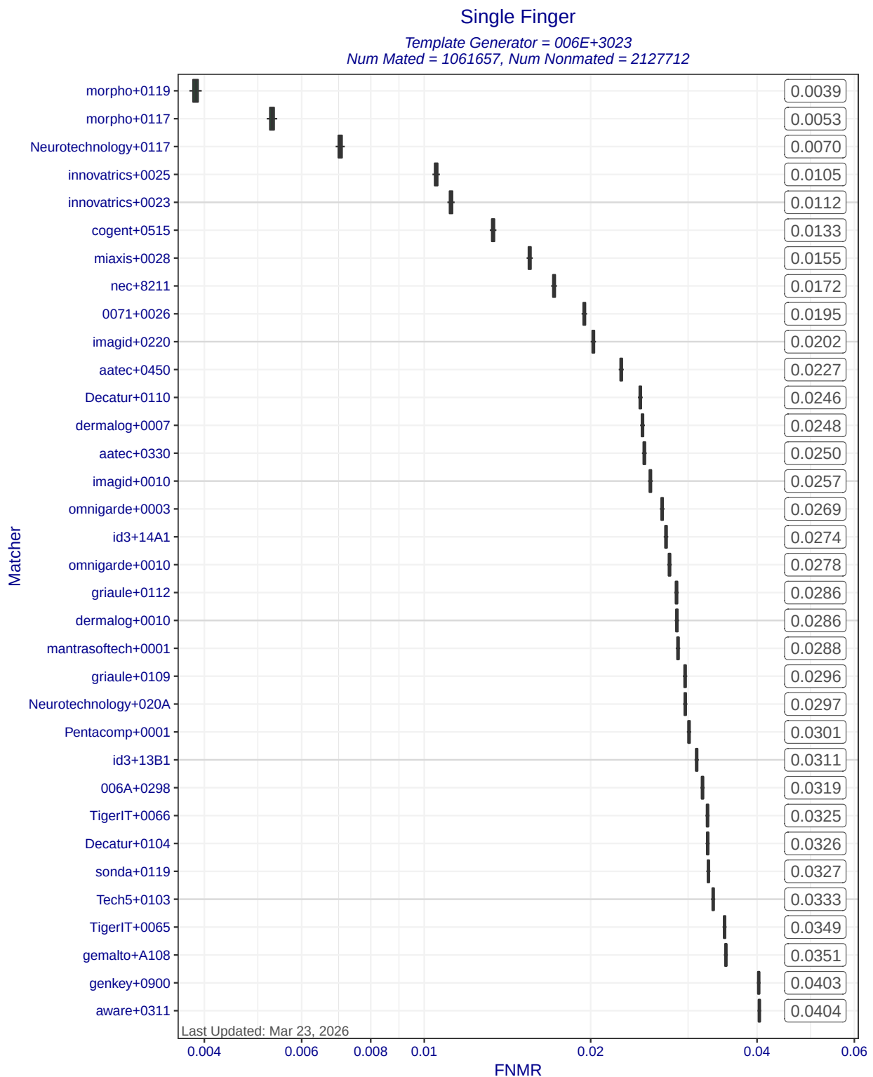
Figure 5: Single Finger FNMRs at FMR=0.0001 when MINEX III compliant matchers compare templates created by template generator 006E+3023. Each box represents uncertainty about the true FNMR. The box edges mark the 50% confidence intervals while the whiskers mark the 90% confidence intervals. The numbers on the right show the actual computed FNMRs.
