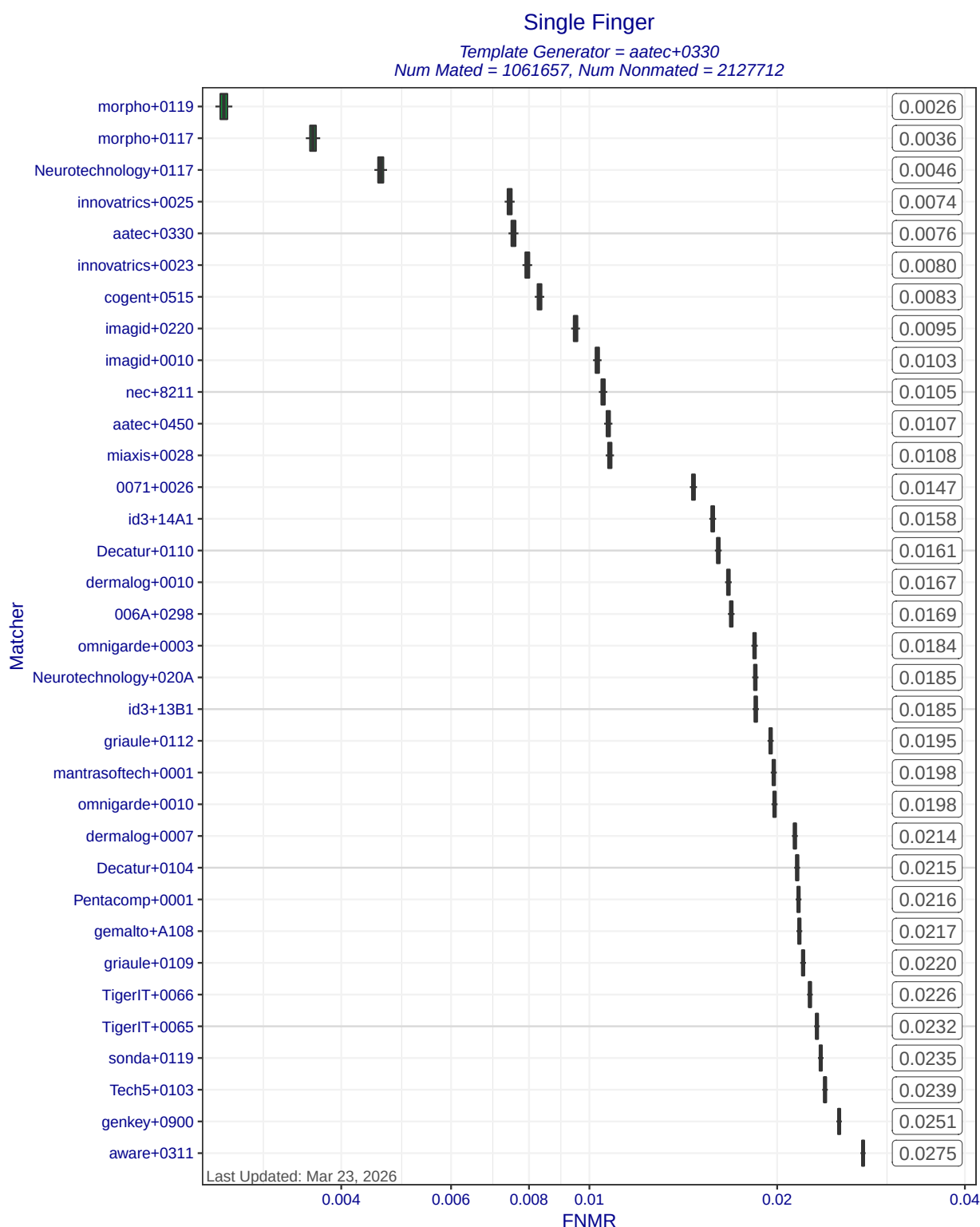
Figure 5: Single Finger FNMRs at FMR=0.0001 when MINEX III compliant matchers compare templates created by template generator aatec+0330. Each box represents uncertainty about the true FNMR. The box edges mark the 50% confidence intervals while the whiskers mark the 90% confidence intervals. The numbers on the right show the actual computed FNMRs.
