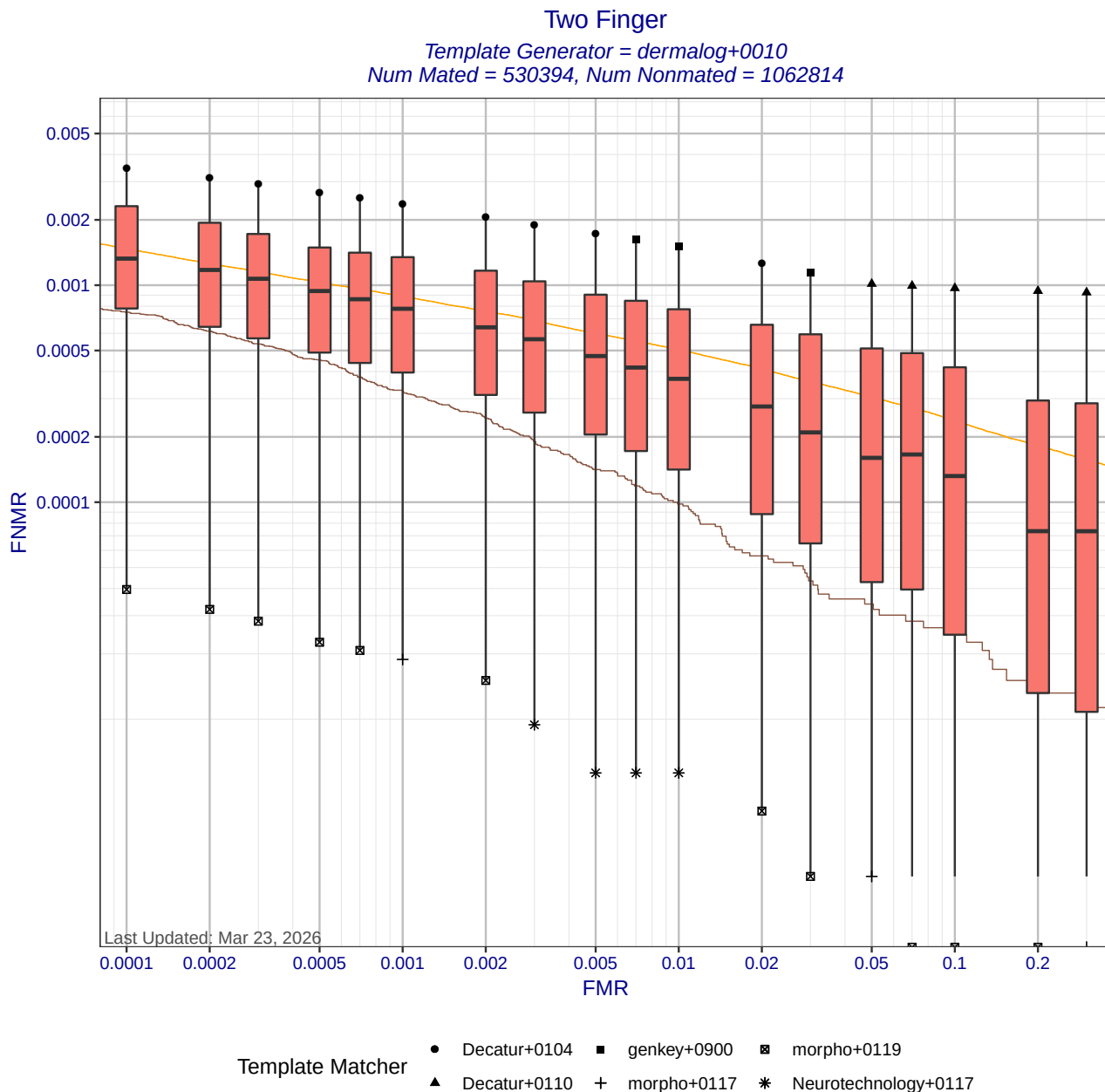
Figure 6: Two Finger DET statistics for template generator dermalog+0010. Each box shows the distribution of FNRs at a fixed FMR across different matchers. The whisker ends show the minimum and maximum FNRs. The brown curve shows the DET curve when the matcher and template generators were submitted by the same participant. The orange DET curve shows pooled performance when all matchers use templates created by dermalog+0010. Score-level fusion is achieved by averaging the scores for left and right index fingers.
