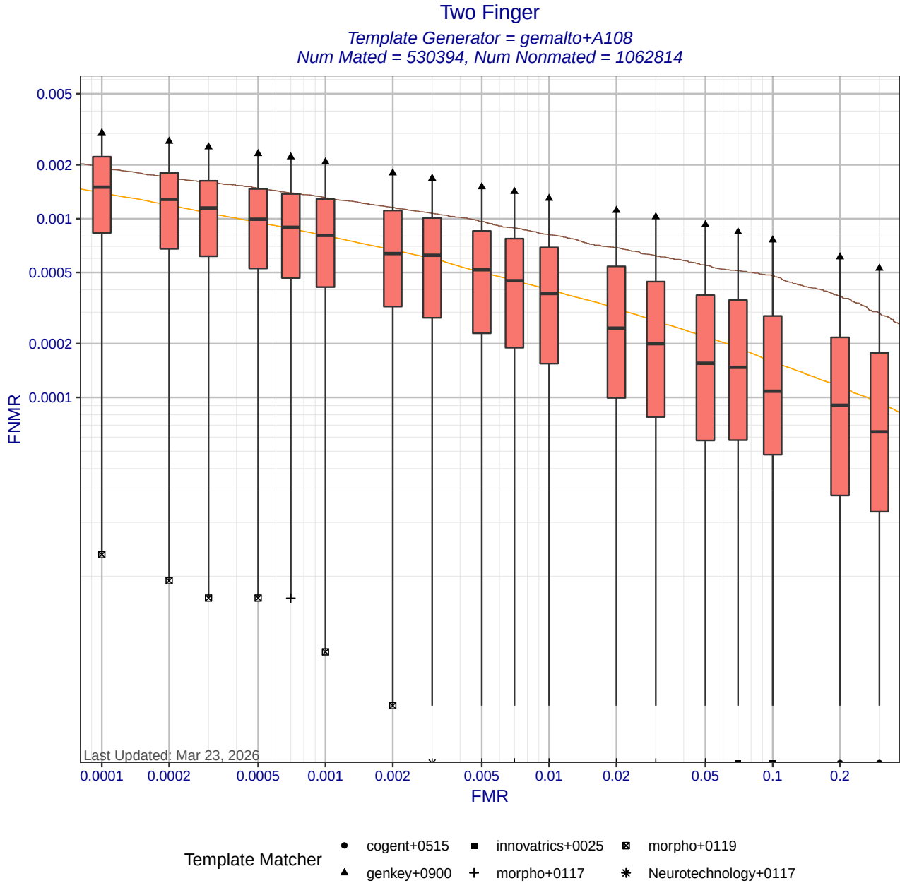
Figure 6: Two Finger DET statistics for template generator gemalto+A108. Each box shows the distribution of FNMNRs at a fixed FMR across different matchers. The whisker ends show the minimum and maximum FNMNRs. The brown curve shows the DET curve when the matcher and template generators were submitted by the same participant. The orange DET curve shows pooled performance when all matchers use templates created by gemalto+A108. Score-level fusion is achieved by averaging the scores for left and right index fingers.
