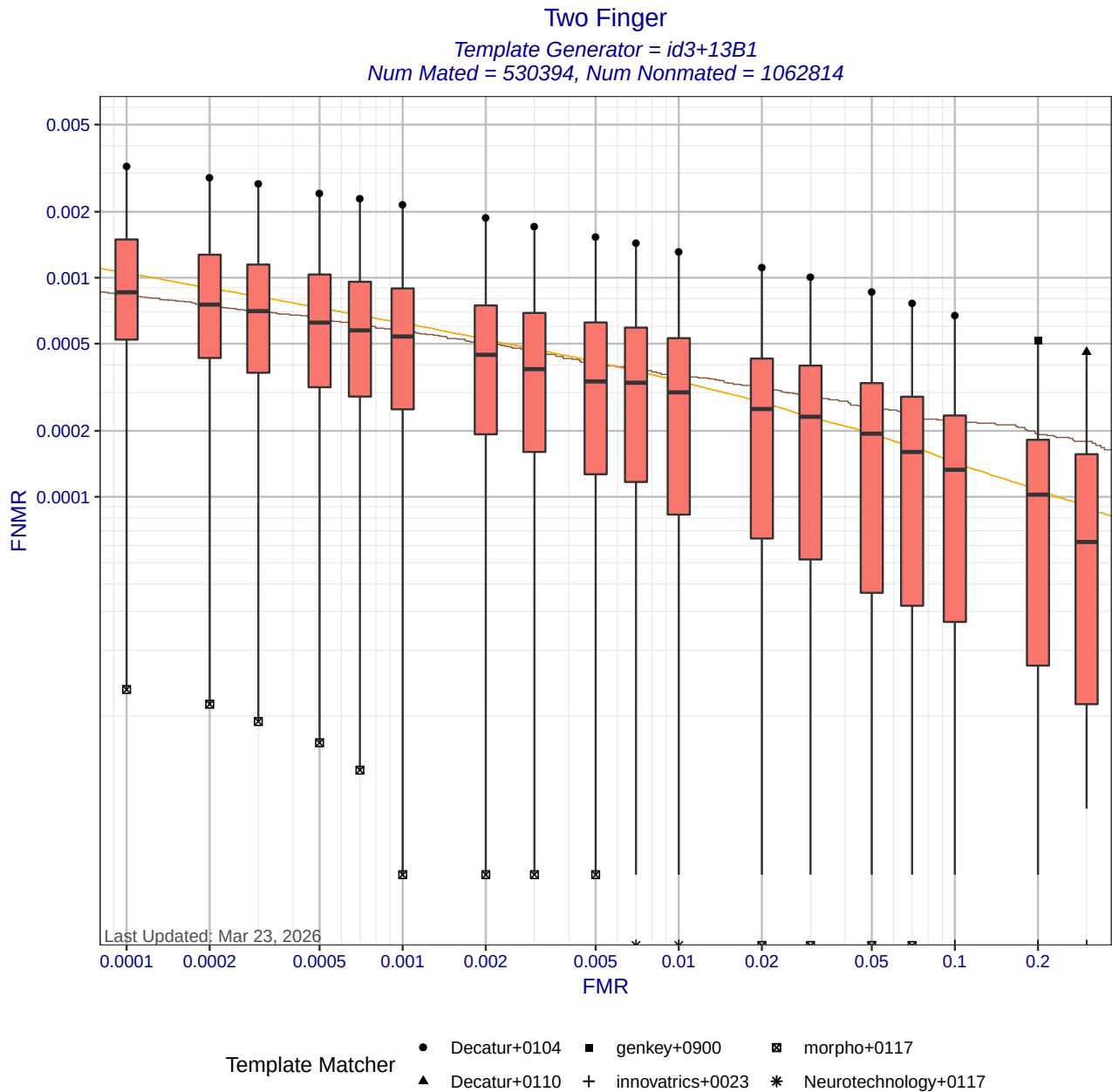
Figure 6: Two Finger DET statistics for template generator id3+13B1. Each box shows the distribution of FNRs at a fixed FMR across different matchers. The whisker ends show the minimum and maximum FNRs. The brown curve shows the DET curve when the matcher and template generators were submitted by the same participant. The orange DET curve shows pooled performance when all matchers use templates created by id3+13B1. Score-level fusion is achieved by averaging the scores for left and right index fingers.
