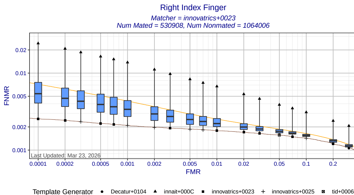
Figure 3: Right index finger DET statistics for matcher innovatrics+0023. Each box shows the distribution of FNMR at a fixed FMR across all MINEX III compliant template generators. The ends of the whiskers show the minimum and maximum FNMRs. The orange DET curve shows pooled performance against all template generators.
