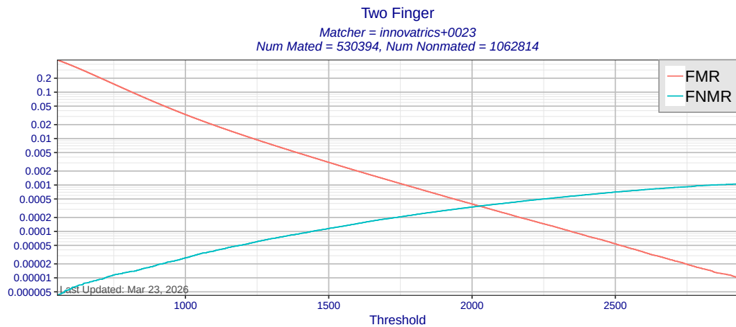
Figure 12: Two finger FMR and FNMR as a function of score threshold for matcher innovatrics+0023 using templates created by all MINEX III compliant template generators. Score-level fusion is achieved by averaging scores for the left and right index fingers.
