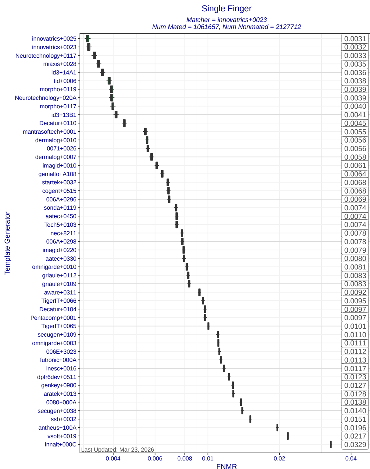
Figure 5: Single finger FNMRs at FMR = 0.0001 when matcher innovatrics+0023 compares templates created by different template generators. The ends of the whiskers show the minimum and maximum FNMRs. Each box represents uncertainty about the true FNMR. The box edges mark the 50% confidence intervals while the whiskers mark the 90% confidence intervals. The numbers on the right show the actual computed FNMRs.
