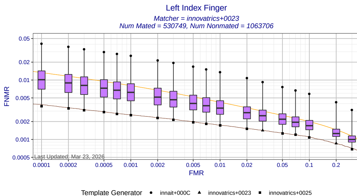
Figure 4: Left index finger DET statistics for matcher innovatrics+0023. Each box shows the distribution of FNMRs at a fixed FMR across all MINEX III compliant template generators. The ends of the whiskers show the minimum and maximum FNMRs. The orange DET curve shows pooled performance against all template generators.
