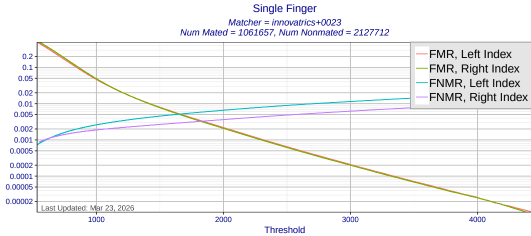
Figure 11: Single finger FMR and FNMR as a function of score threshold for matcher innovatrics+0023 using templates created by all MINEX III compliant template generators. Separate curves are presented for left and right index fingers.
