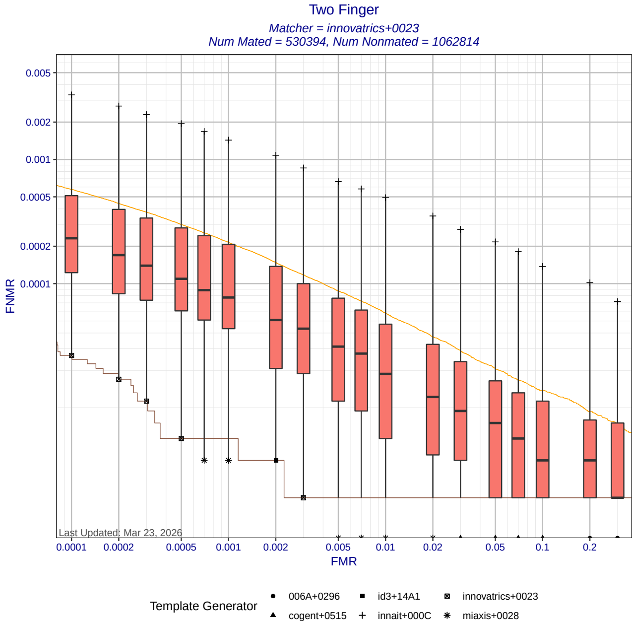
Figure 7: Two finger DET statistics for matcher innovatrics+0023. Each box shows the distribution of FNMRs at a fixed FMR across all MINEX III compliant template generators. The whisker ends show the minimum and maximum FNMRs. The orange DET curve shows pooled performance against all template generators. Score-level fusion is achieved by averaging the scores for left and right index fingers.
