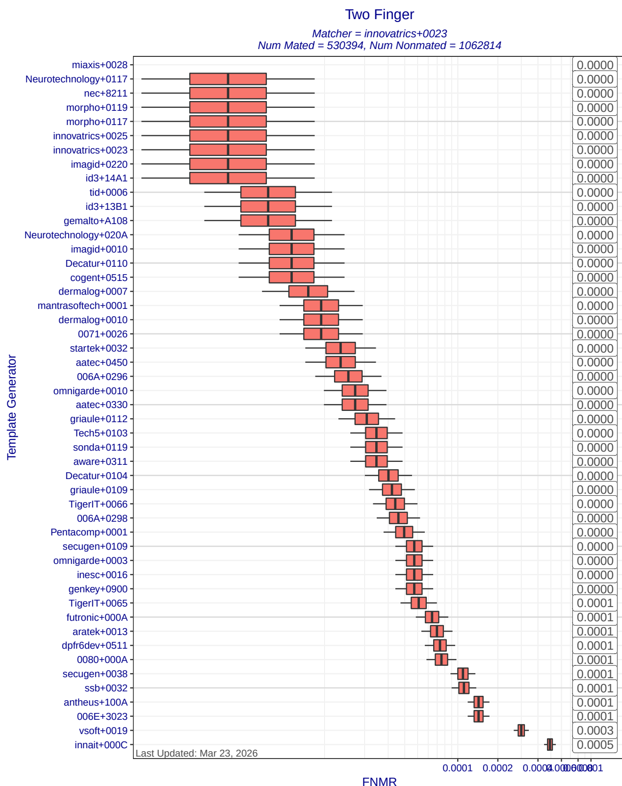
Figure 8: Two finger FNMR at FMR=0.01 when matcher innovatrics+0023 compares templates created by different template generators. Each box represents uncertainty about the true FNMR. The box edges mark the 50% confidence intervals while the whiskers mark the 90% confidence intervals. The numbers on the right show the actual computed FNMRs. Score-level fusion is achieved by averaging the scores for left and right index fingers.
