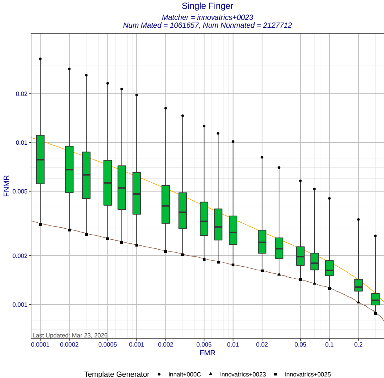
Figure 2: Single finger DET statistics for matcher innovatrics+0023. Each box shows the distribution of FNMRs at a fixed FMR across all MINEX III compliant template generators. The ends of the whiskers show the minimum and maximum FNMRs. The orange DET curve shows pooled performance against all template generators.
