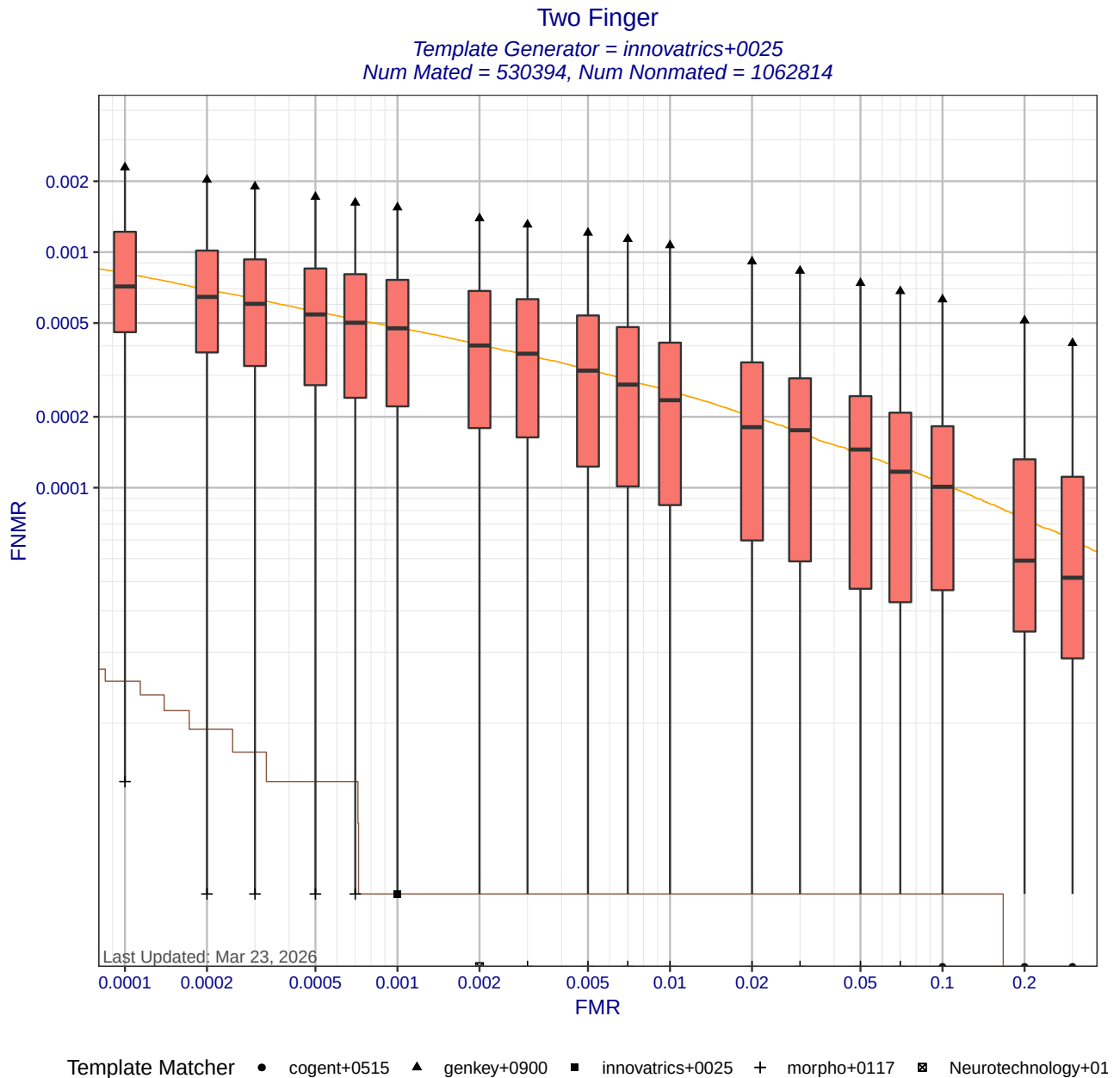
Figure 6: Two Finger DET statistics for template generator innovatrics+0025. Each box shows the distribution of FNMNRs at a fixed FMR across different matchers. The whisker ends show the minimum and maximum FNMNRs. The brown curve shows the DET curve when the matcher and template generators were submitted by the same participant. The orange DET curve shows pooled performance when all matchers use templates created by innovatrics+0025. Score-level fusion is achieved by averaging the scores for left and right index fingers.
