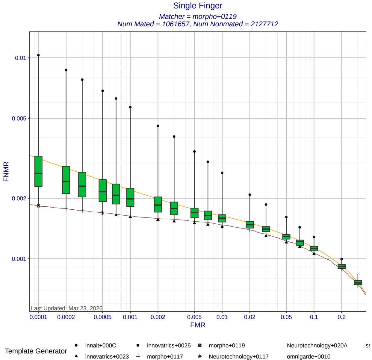
Figure 2: Single finger DET statistics for matcher morpho+0119. Each box shows the distribution of FNMRs at a fixed FMR across all MINEX III compliant template generators. The ends of the whiskers show the minimum and maximum FNMRs. The orange DET curve shows pooled performance against all template generators.
